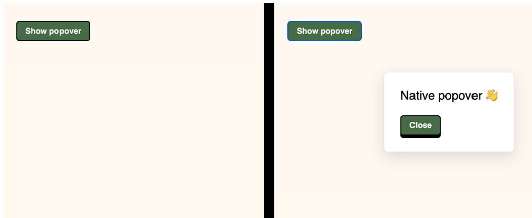
Figure 15.1 - Final result: Left - no popover. Right - a showing popover.
