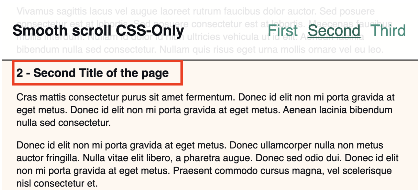
Figure 3.2 - Section title with offset.
