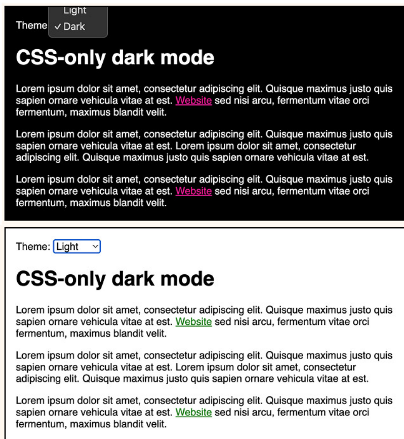
Figure 2.1 - Final result: Darkmode on the left. Lightmode on the right.
