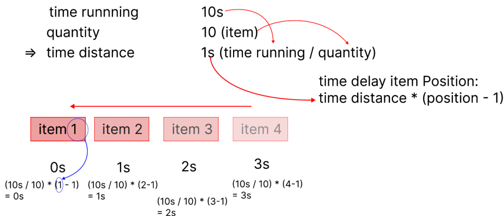
Figure 6.2 - Alternative explanation of the formula.
