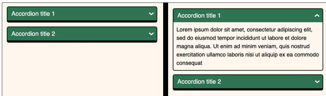
Figure 5.3 - Example of a finished accordion.
