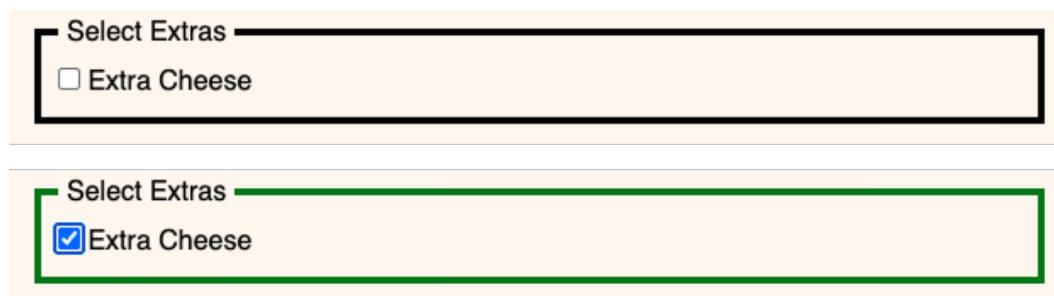
Figure 1.1 - Final result: change color of fieldset when input is checked.
