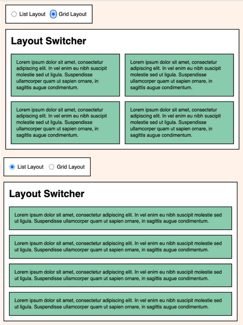
Figure 1.5 - Final result: Change the display of your content by checking a checkbox.
