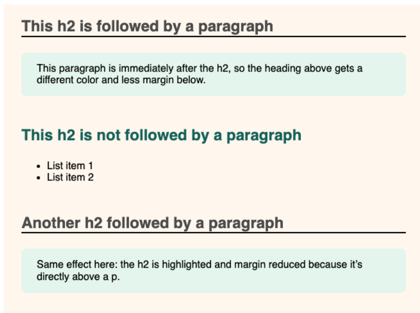
Figure 1.4 - Final result: second title is different because it has no paragraph.
