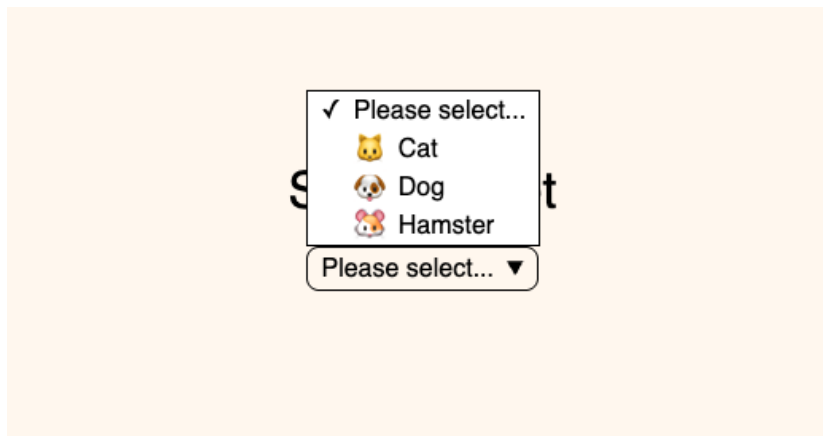
Figure 16.2 - Result with just this line of CSS.
