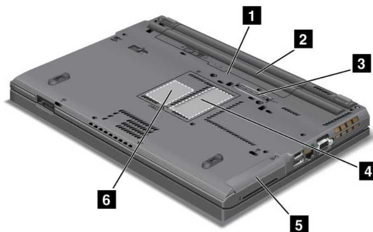
Figure 4. ThinkPad T420/T420i bottom view
