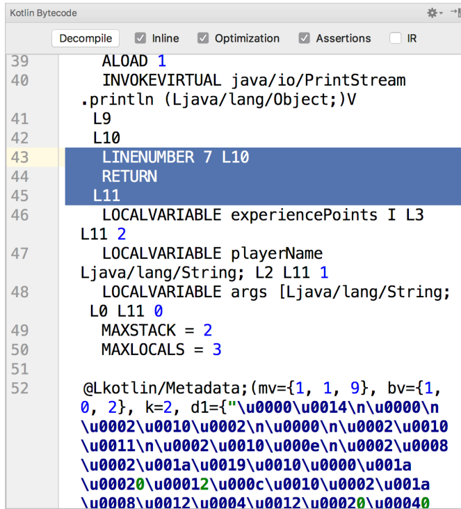
Figure 2.10 Kotlin bytecode tool window
