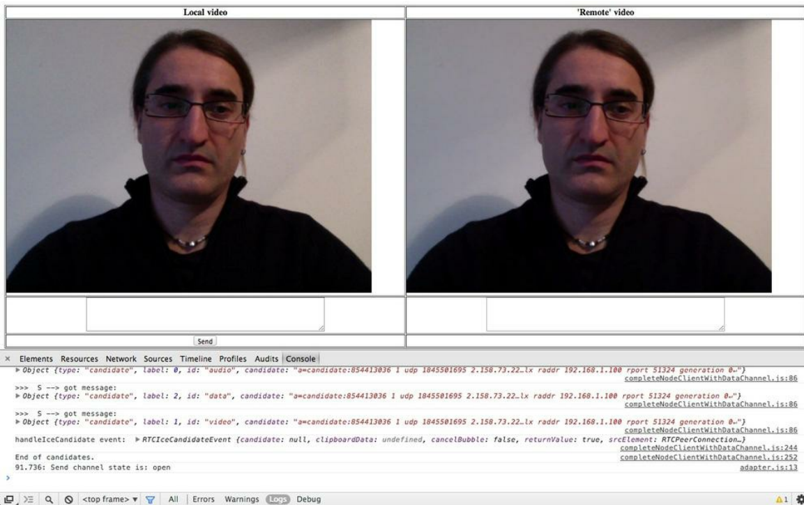
Figure 5-18. Communication established in Chrome: Initiator's side
