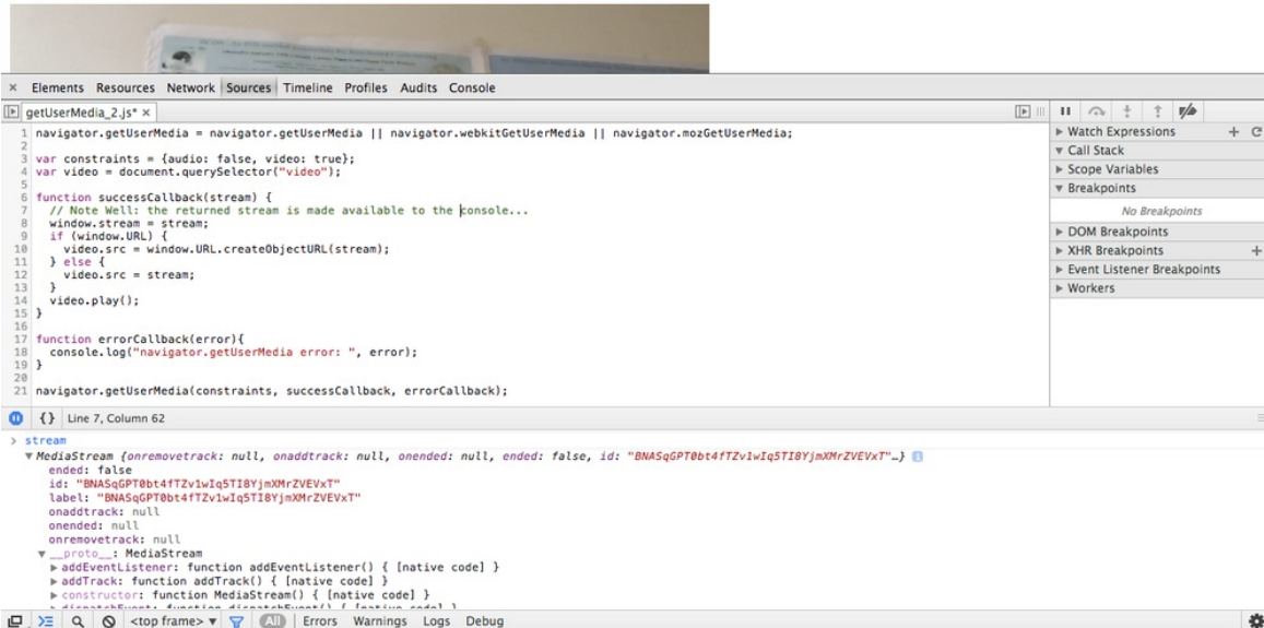
Figure 2-6. Inspecting a MediaStream in Chrome's console
