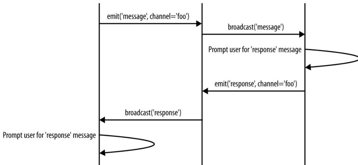
Figure 4-11. Starting a conversation
