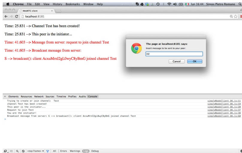
Figure 4-10. Starting a conversation after channel setup
