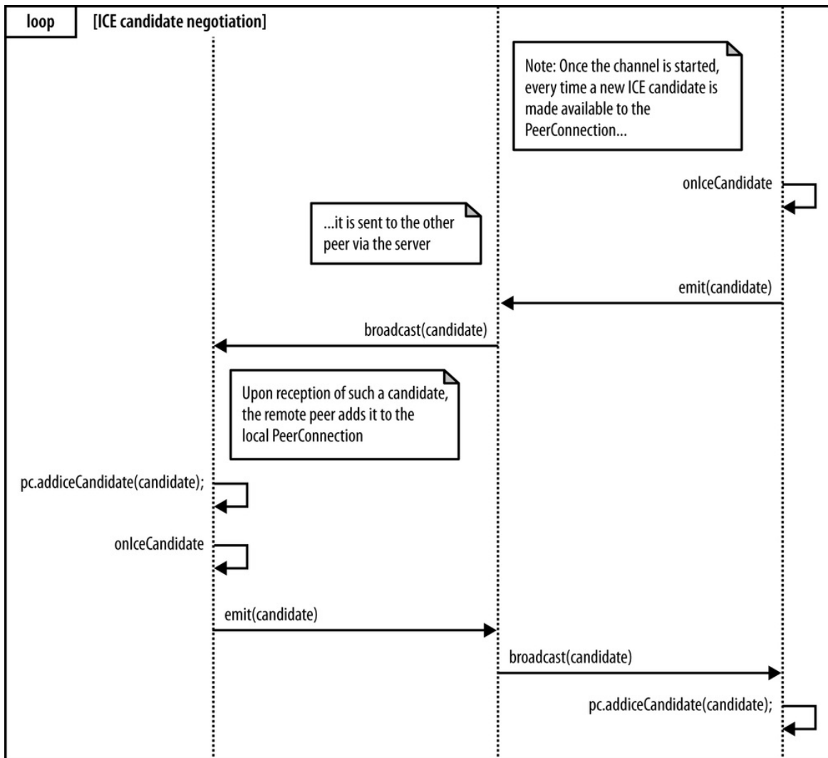
Figure 5-13. Server-mediated ICE candidate exchange procedure
