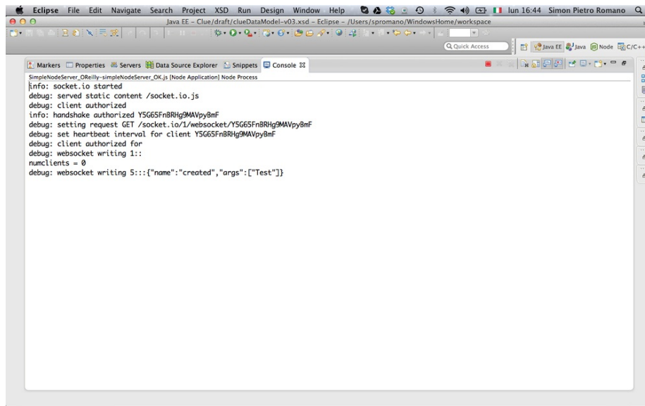
Figure 4-4. Signaling server managing initiator's request
