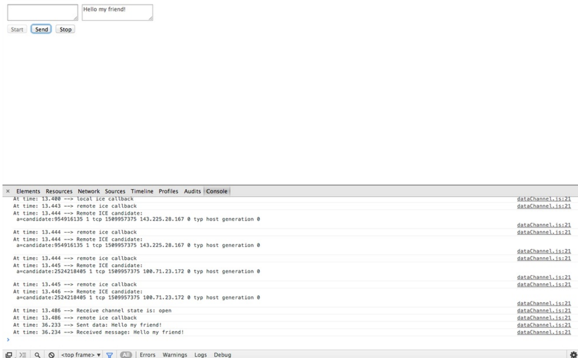
Figure 3-19. Receiving a message from the data channel in Chrome
