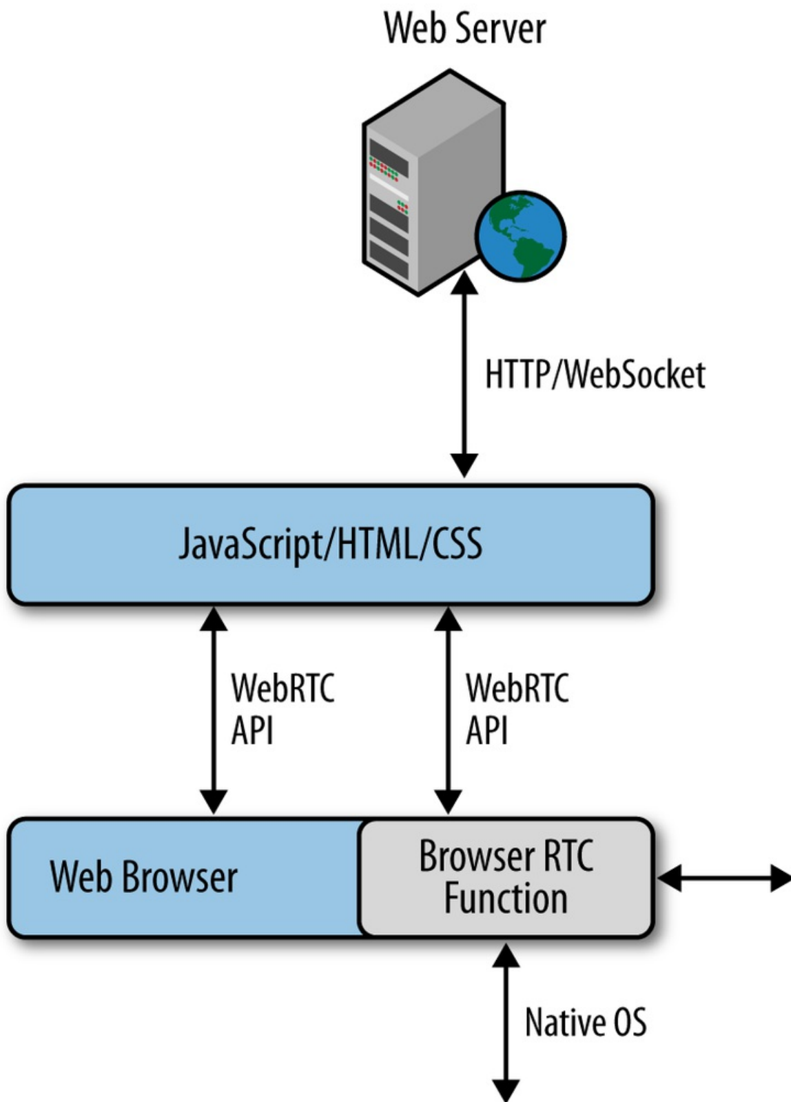
Figure 1-3. Real-time communication in the browser
