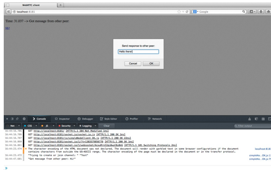
Figure 4-13. Remote peer receiving relayed message from signaling server
