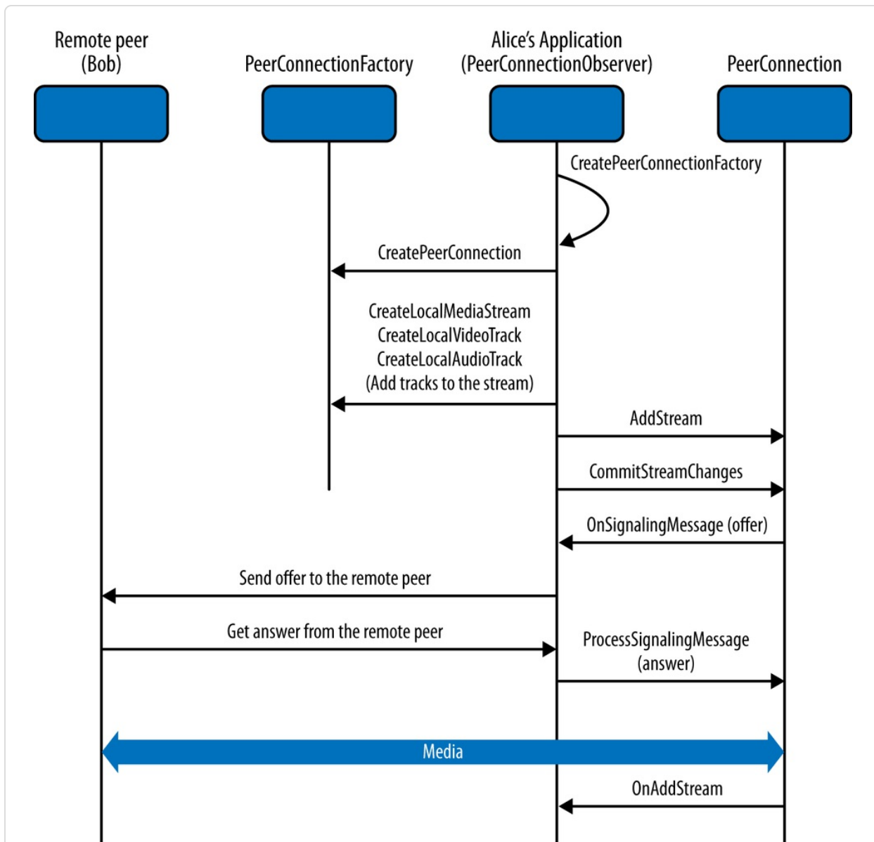
Figure 1-5. Call setup from Alice's perspective
