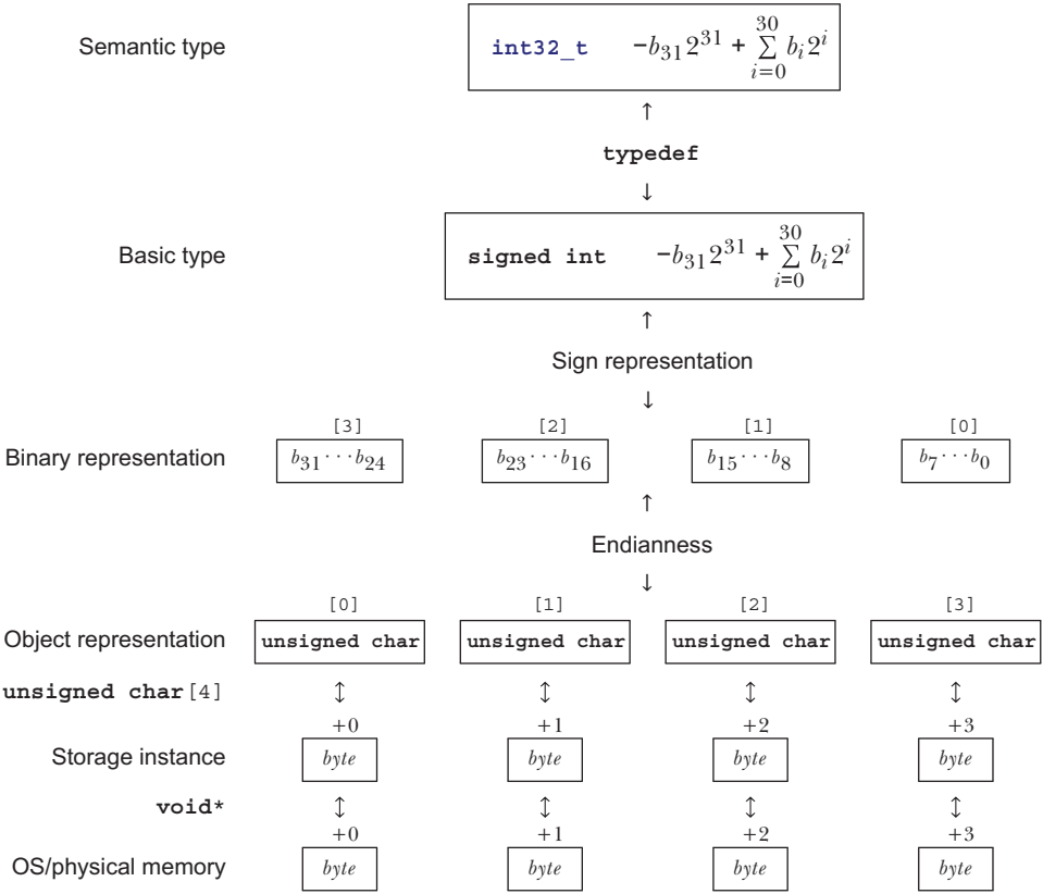
Figure 12.1 The different levels of the value-memory model for an int32_t . Example of a platform that maps this type to a 32-bit signed int and uses a little-endian object representation.
