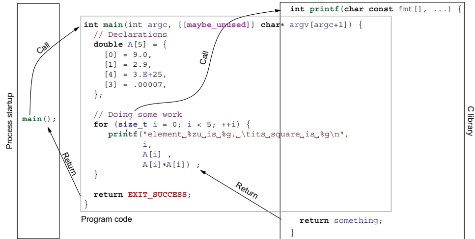
Figure 2.1 Execution of a small program
