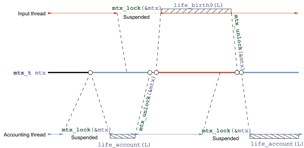
Figure 21.2 Two threads with three critical sections that synchronize via a mutex. The circles present the modifications of object mtx .
