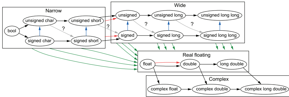
Figure 18.1 Upward conversion of some standard arithmetic types. Black arrows conserve values; red arrows (between narrow and wide types) may occur for integer promotion or default argument conversion; blue arrows (from signed to unsigned types) are reduction modulo 2^N ; well-definition of gray arrows (with question marks) depends on the platform; green arrows (from integers to floating types) may lose precision.
