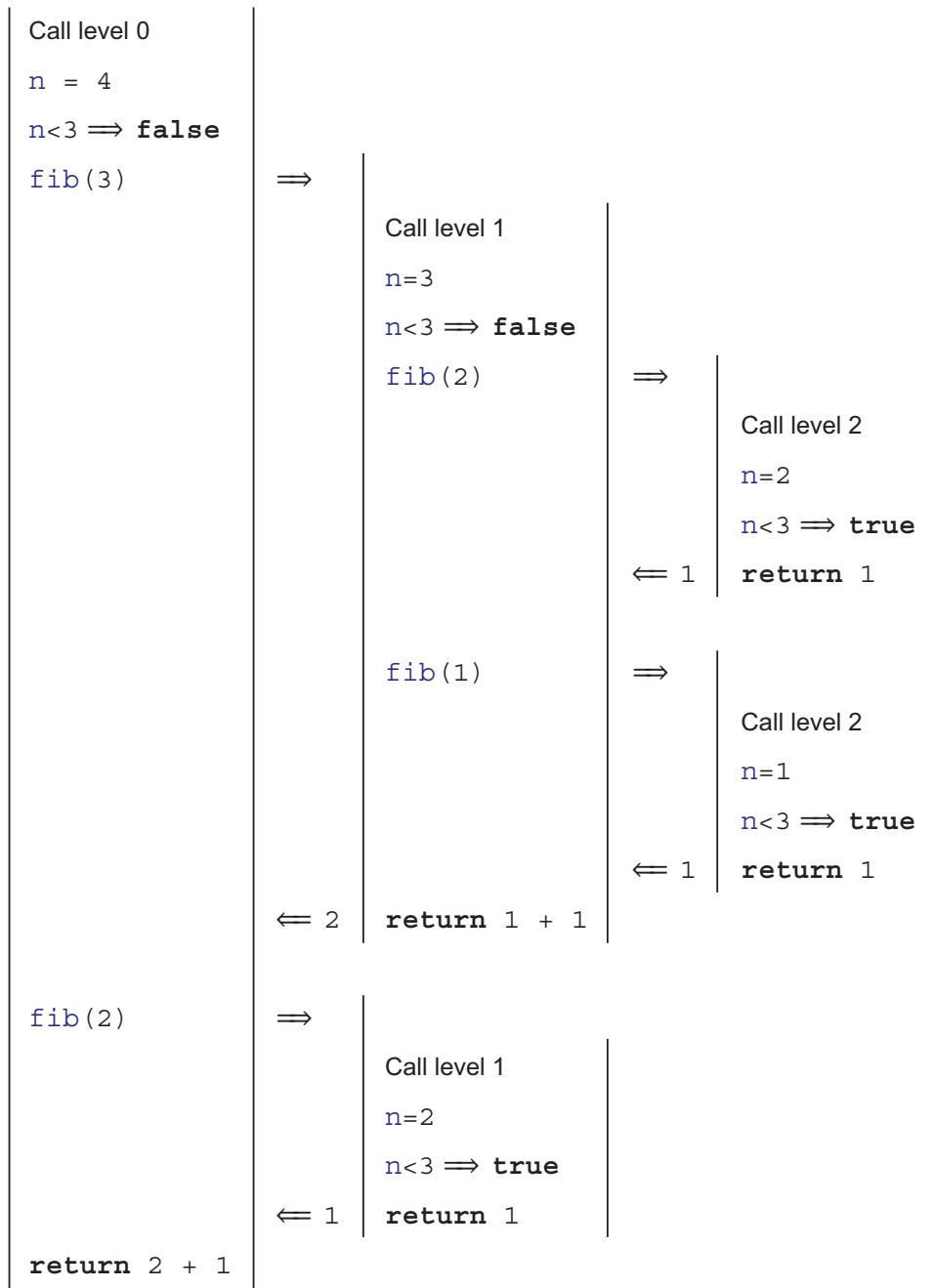
Figure 7.2 Recursive call fib(4)
