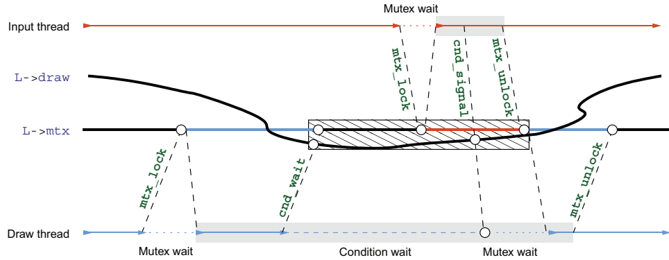
Figure 20.3 Control flow managed by mutex L->mtx and condition variable L->draw between the input and draw threads. Critical sections are shaded with grey. The condition variable is associated with the mutex until the waiter has reacquired the mutex.
