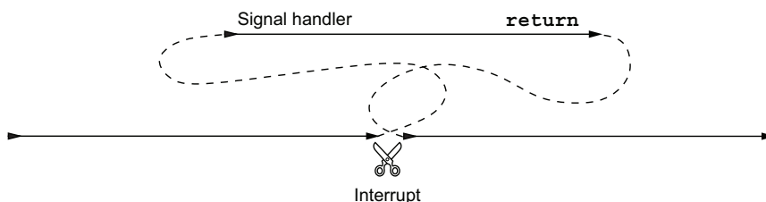
Figure 19.3 Control flow after an interrupt return jumps to the position where the interrupt occurred
