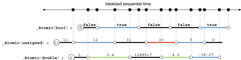
Figure 21.3 Sequential consistency for three different atomic objects
