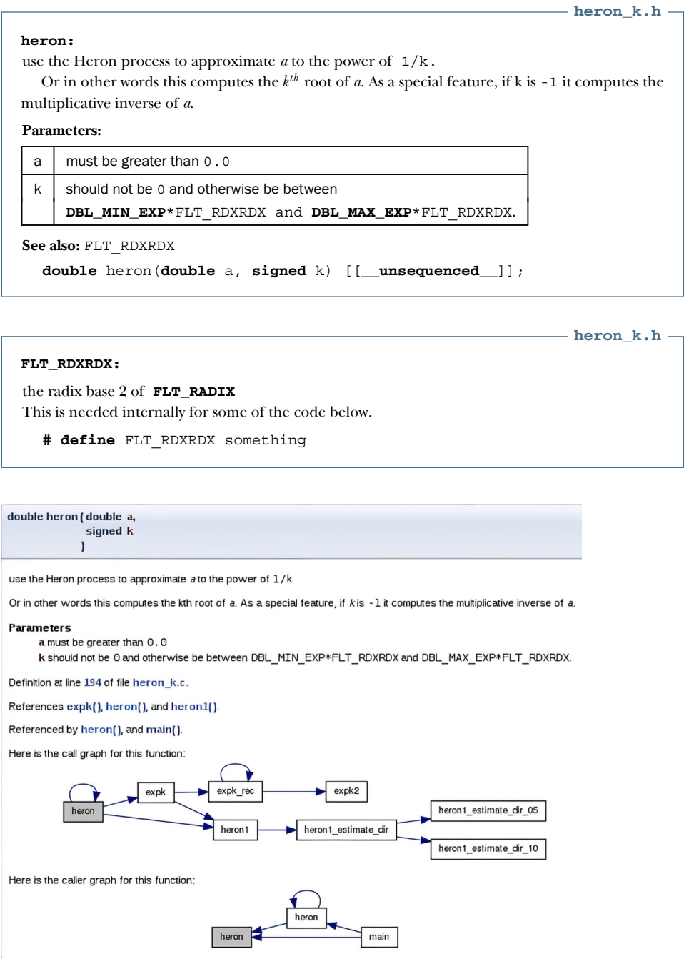
Figure 10.1 Documentation produced by Doxygen
