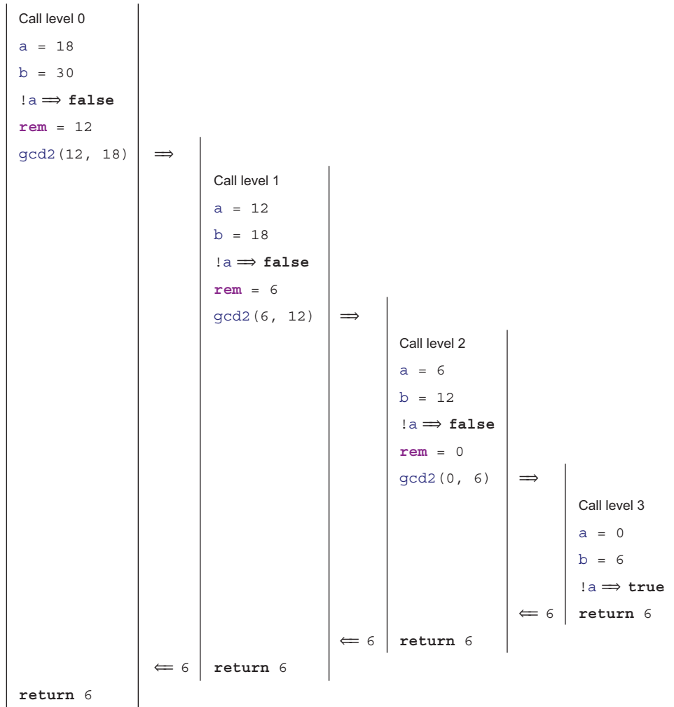
Figure 7.1 Recursive call gcd2(18, 30)
