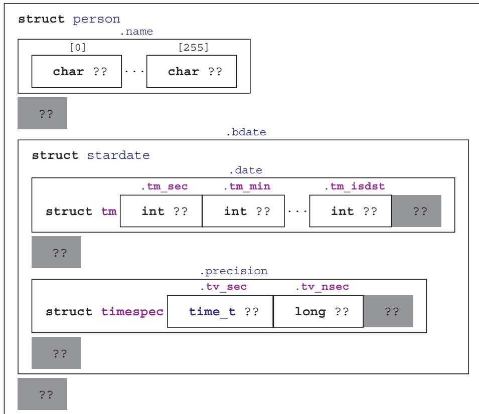
Figure 6.1 A structure layout
