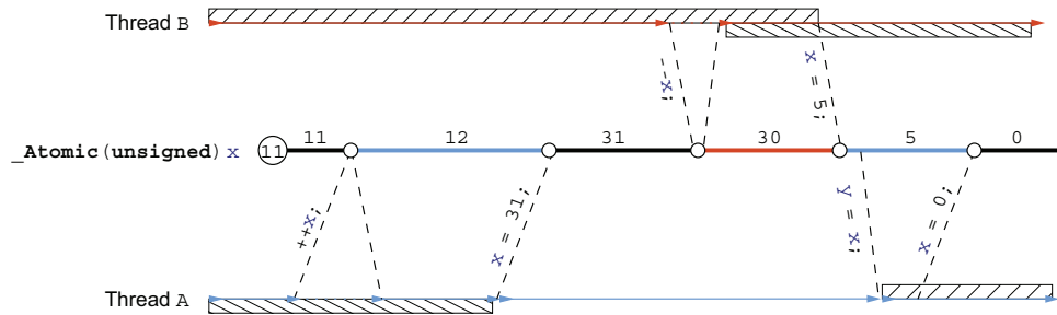
Figure 21.1 Two threads that synchronize via an atomic. The circles present the modifications of object x . The bars below the threads represent information about the state of A , and those above represent information about the state of B .
