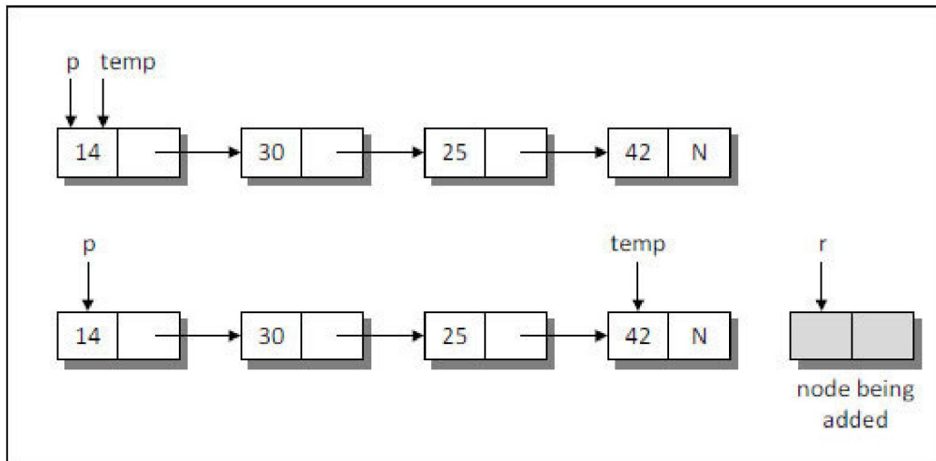
Figure 3-2. Working of append() function.
