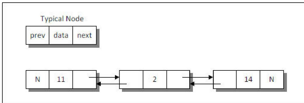
Figure 3-9. Doubly linked list.
