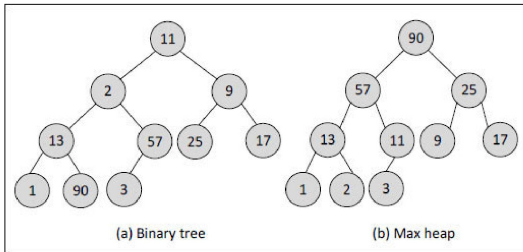
Figure 7-20. Conversion of binary tree to max heap.
