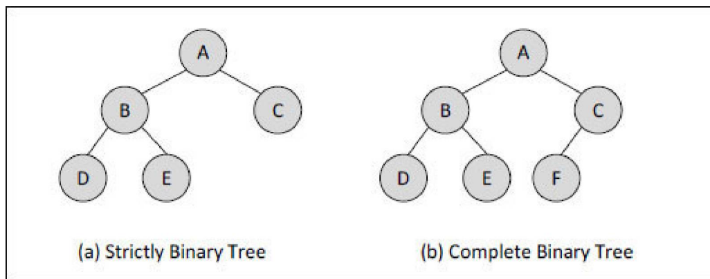
Figure 7-3. Strictly and Complete binary tree.
