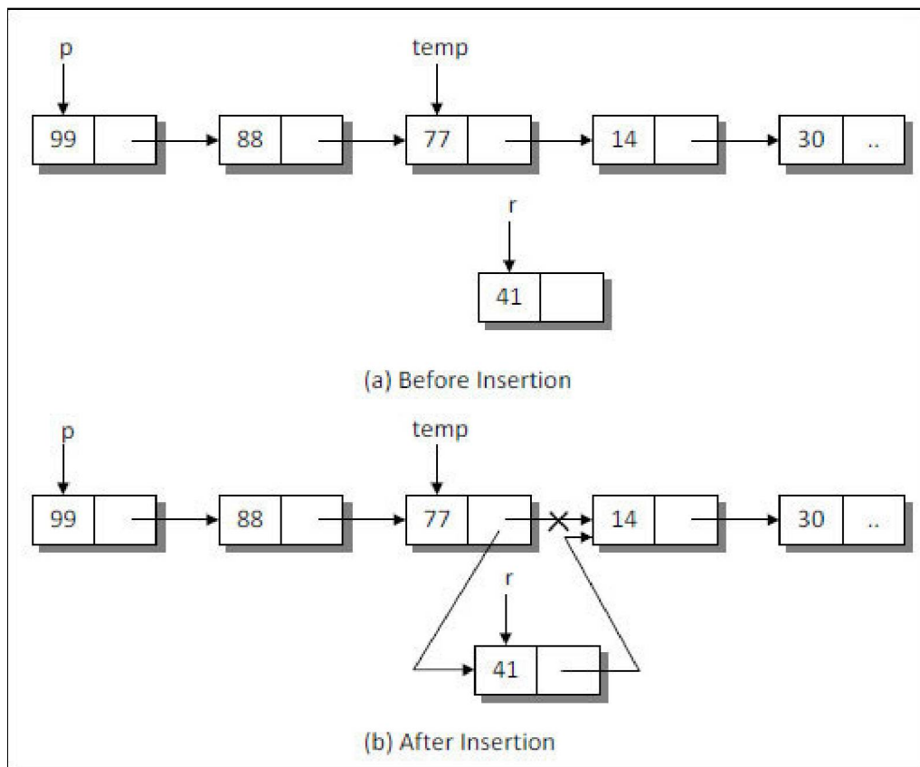
Figure 3-5. Working of addafter() function.
