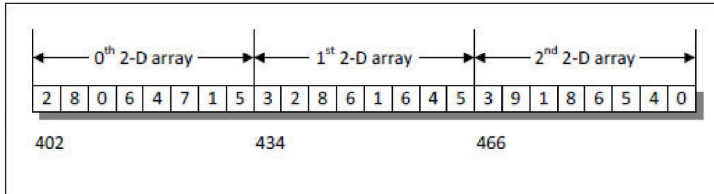
Figure 2-6. Memory representation of a 3-D array.
