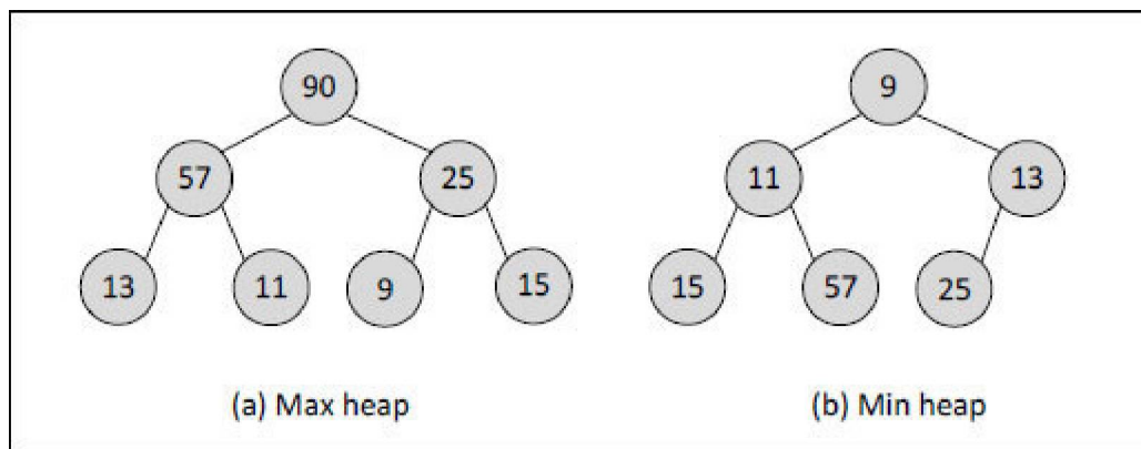
Figure 7-17. Types of heaps.
