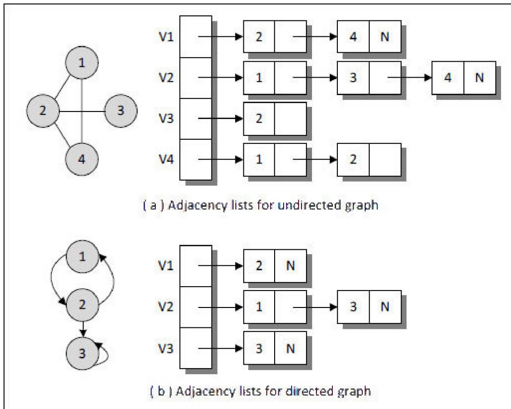
Figure 8-3. Adjacency
