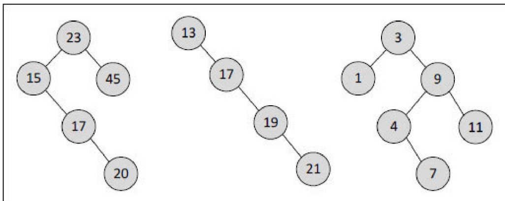
Figure 7-7. Sample BSTs.
