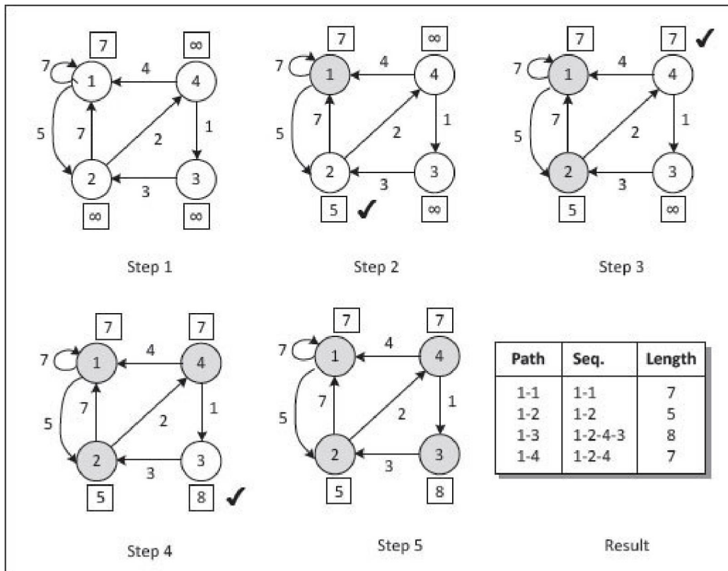
Figure 8-12. Implementation of Dijkstra's algorithm.
