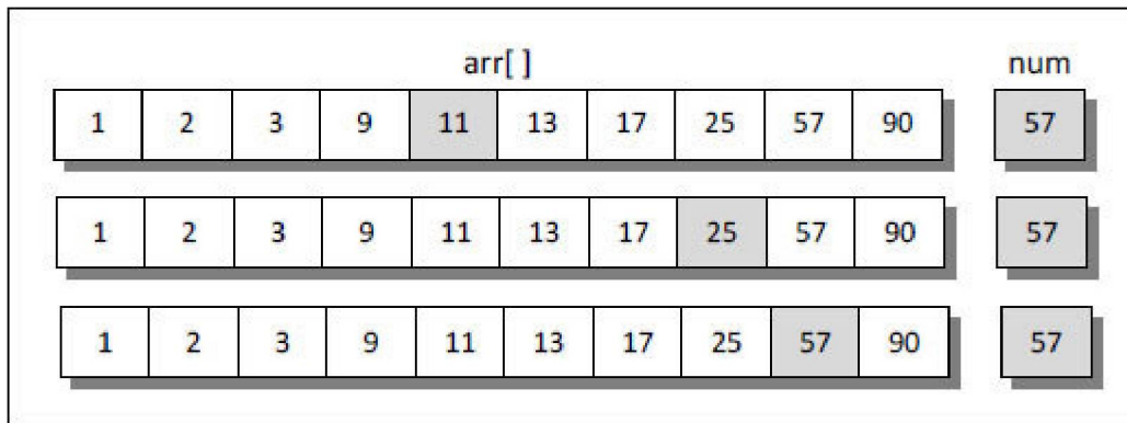
Figure 9-1. Binary
