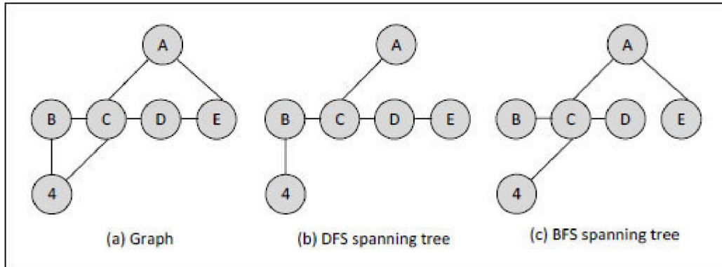
Figure 8-8. Graph and its depth / breadth first search spanning
