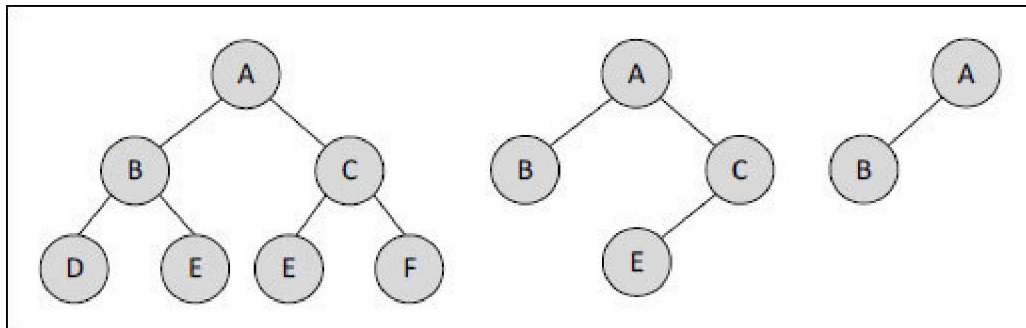
Figure 7-15. AVL trees.
