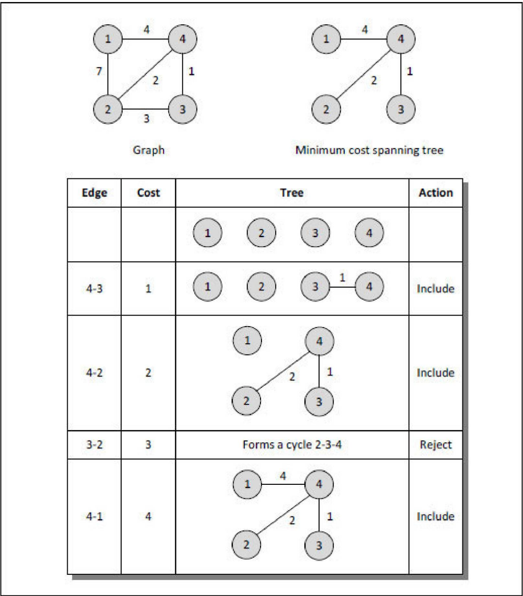
Figure 8-10. Minimum cost spanning tree using Kruskal's algorithm.
