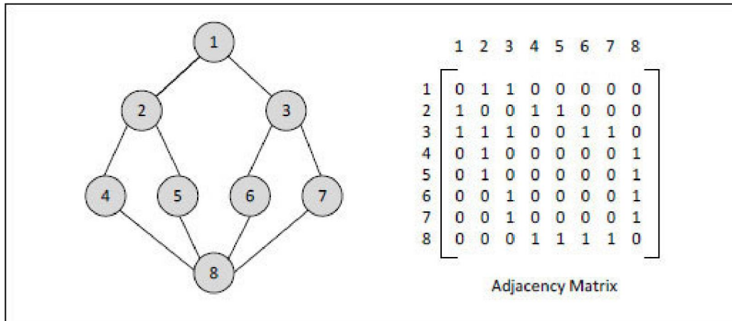
Figure 8-6. Graph and its adjacency
