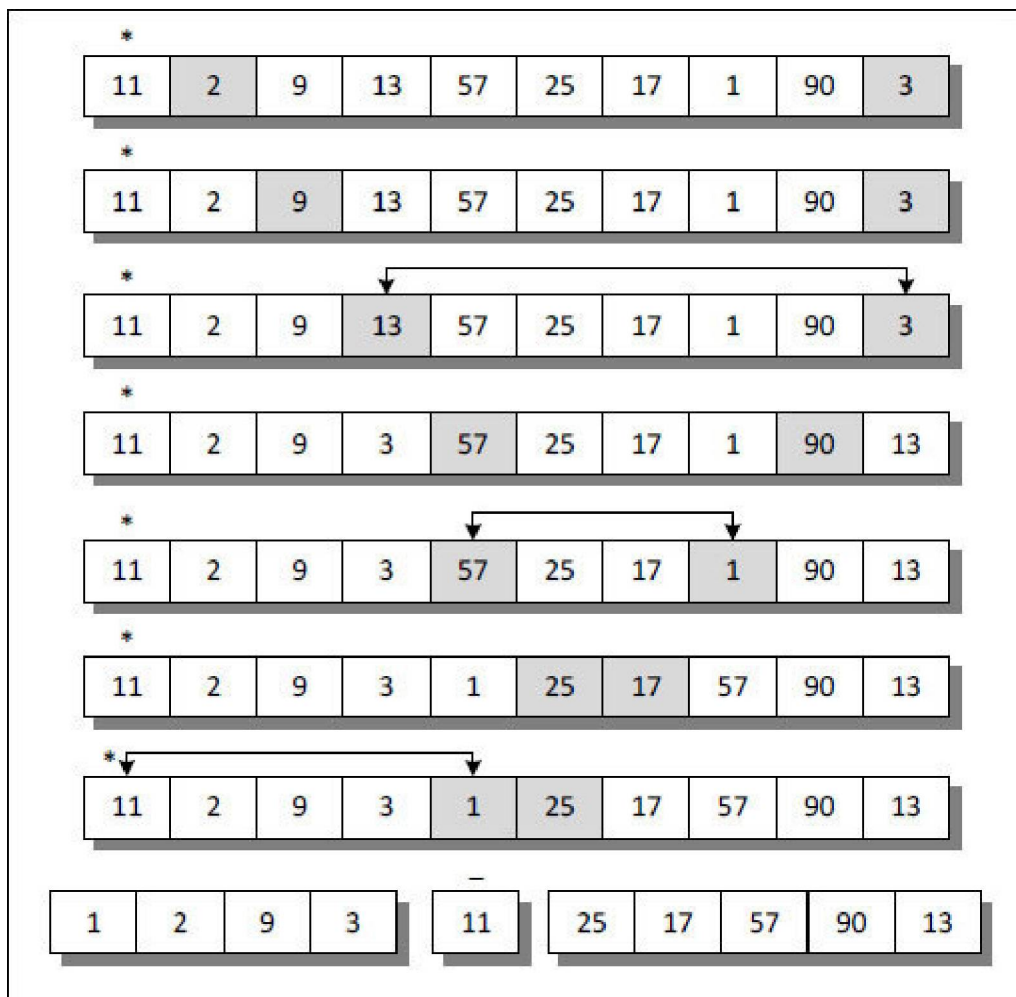
Figure 9-6. Quick
