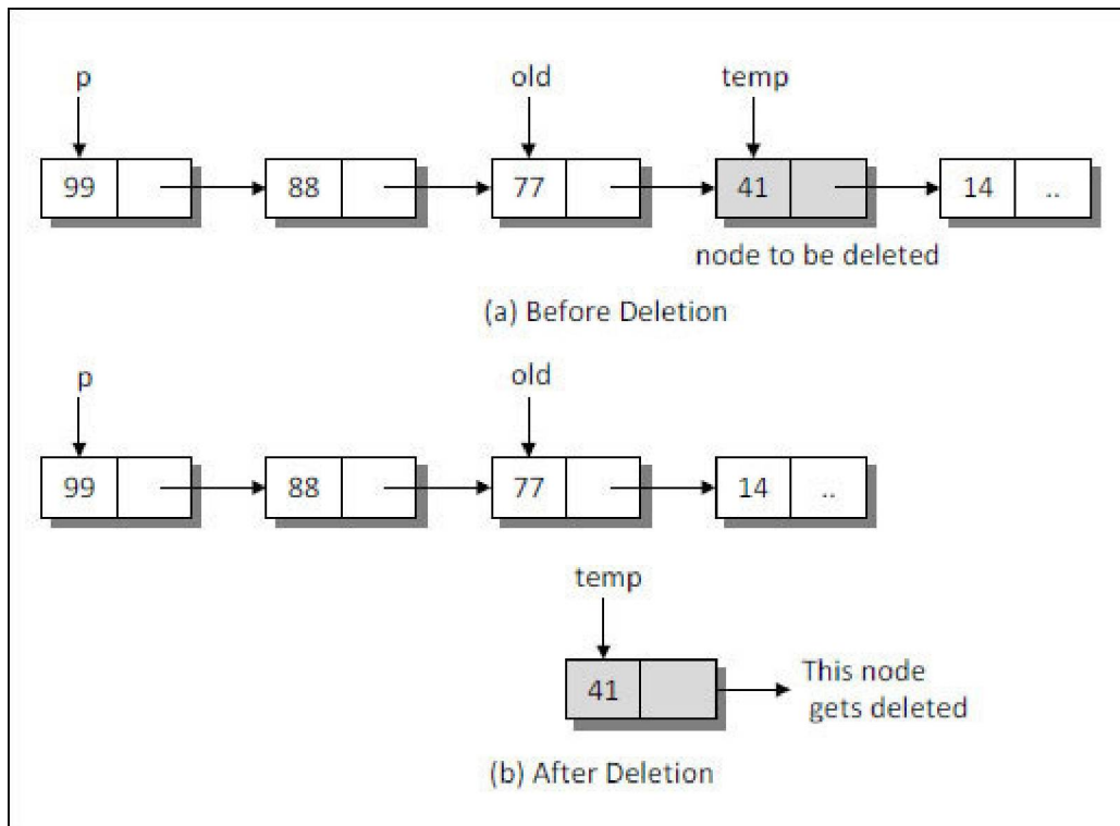
Figure 3-6. Working of del() function.
