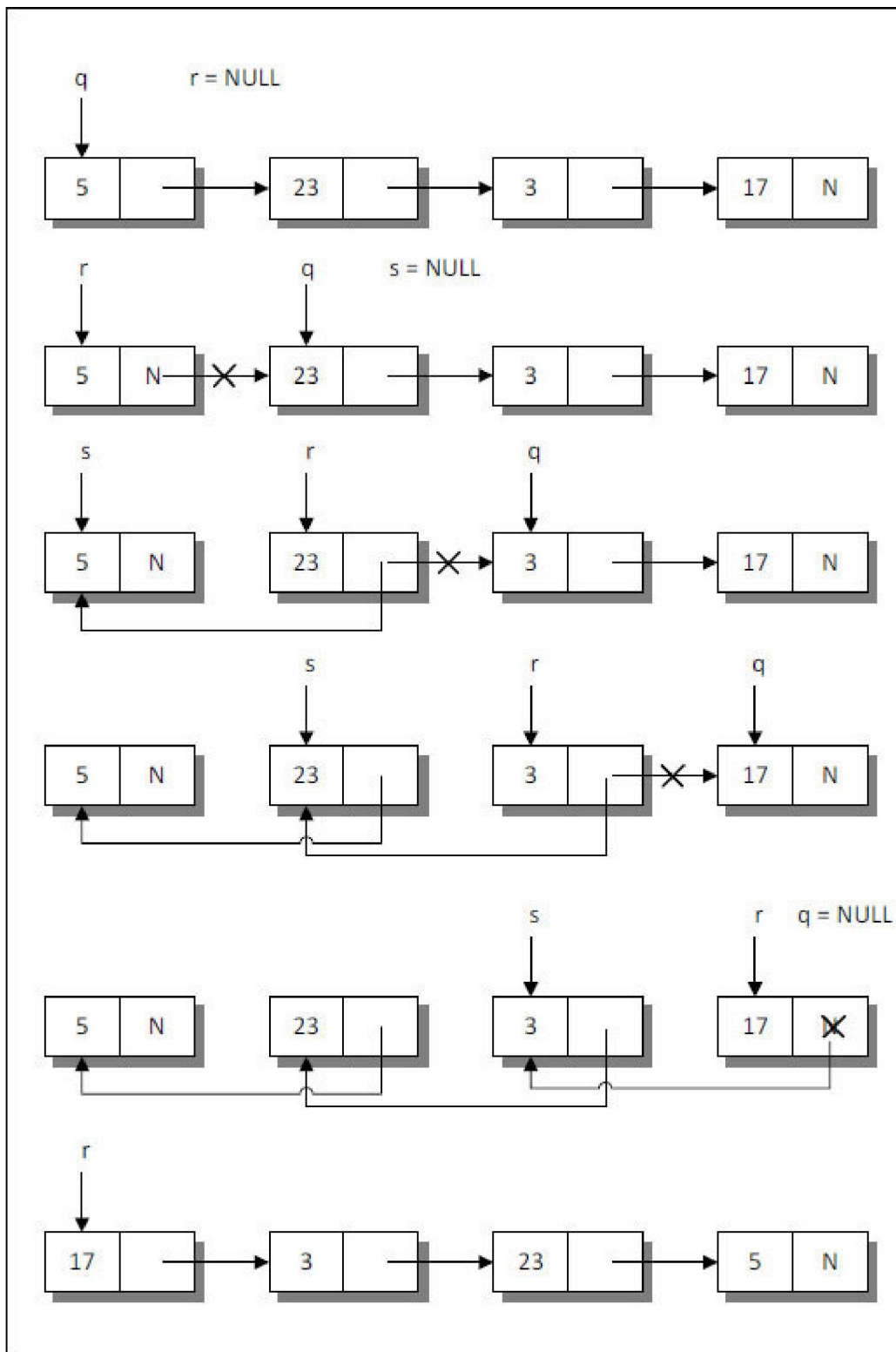
Figure 3-8. Reversing the links.
