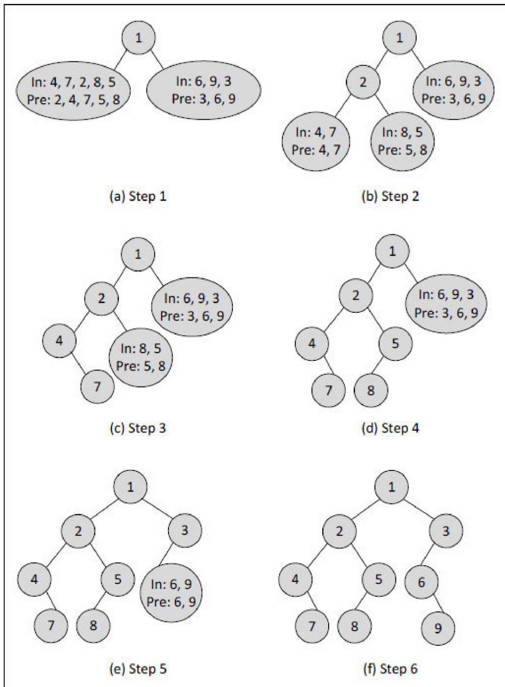
Figure 7-12. Reconstruction of a binary tree.
