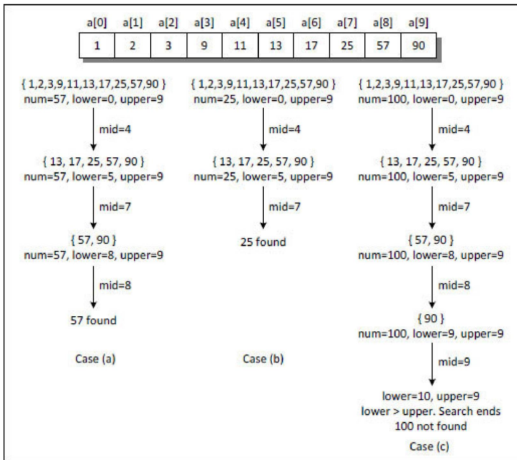
Figure 9-2. Progress of recursive Binary
