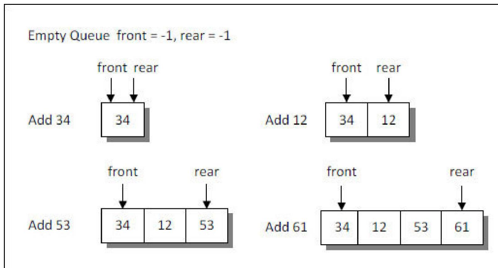
Figure 6-2. Addition of an element to a queue.
