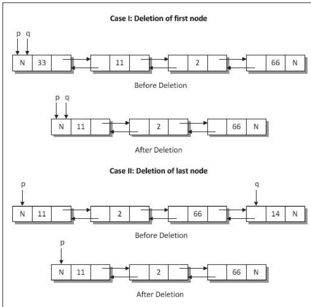
Figure 3-12. Working of d_delete() function.
