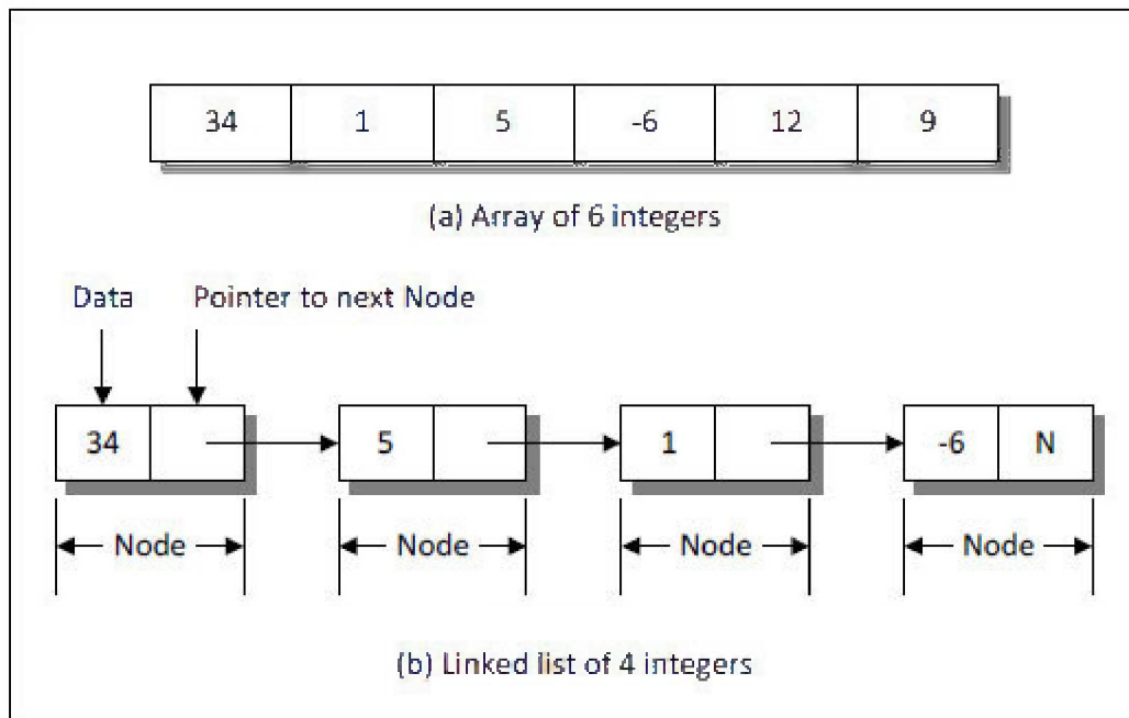
Figure 2-1. Array and Linked list.
