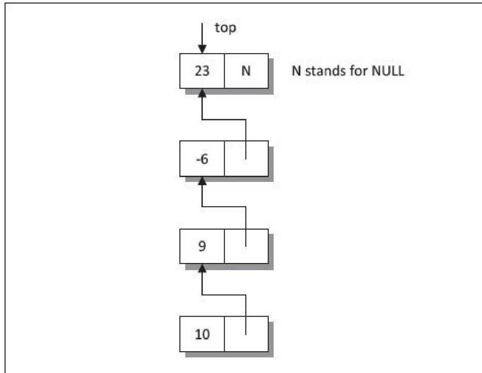
Figure 5-2. Representation of stack as a linked list.
