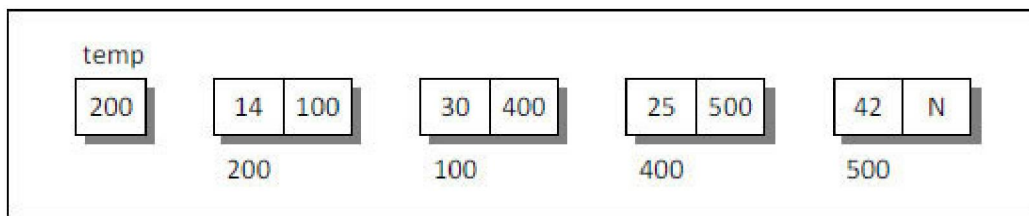
Figure 3-3. Connection of nodes.
