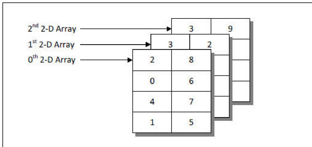
Figure 2-5. Representation of a 3-D array.
