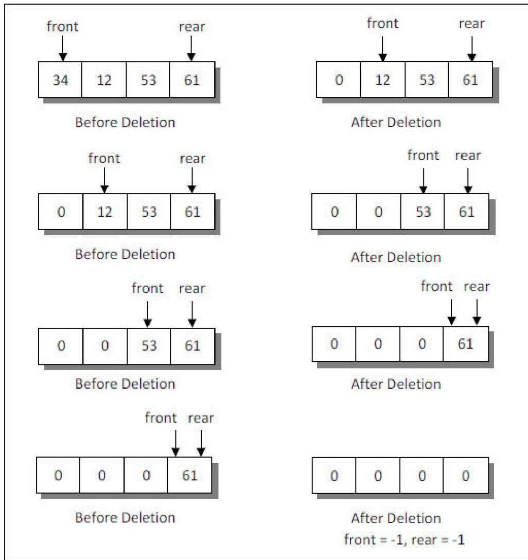
Figure 6-3. Deletion of elements from a queue.
