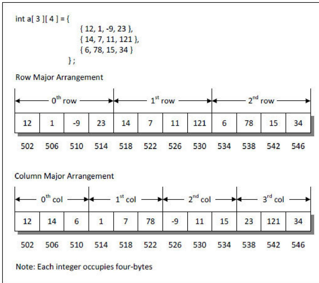
Figure 2-4. Possible arrangements of 2-D array.
