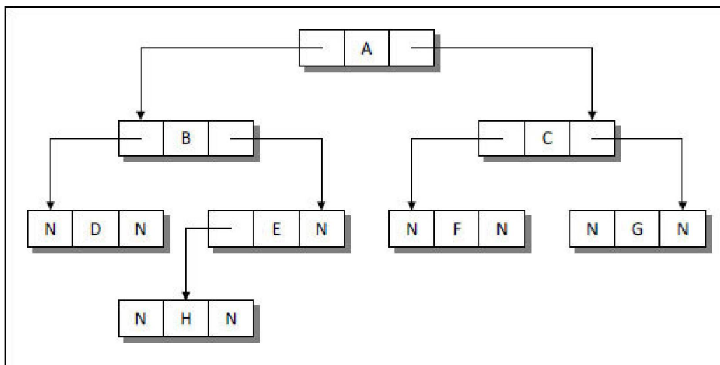
Figure 7-4. Linked representation of a Binary tree.
