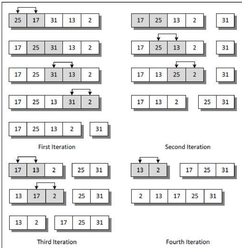
Figure 9-3. Bubble sort at
