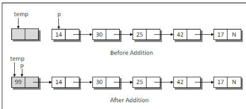
Figure 3-4. Working of addatbeg() function.
