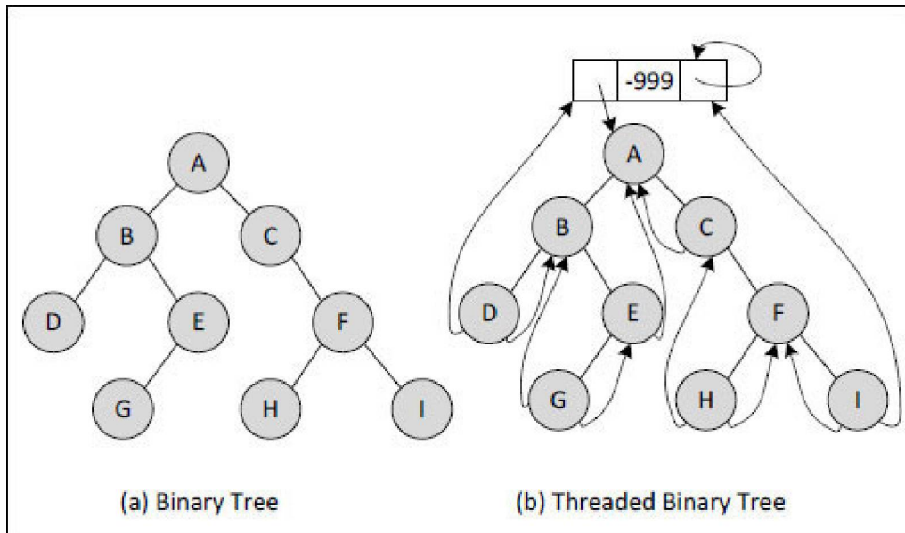
Figure 7-13. Threaded binary tree.
