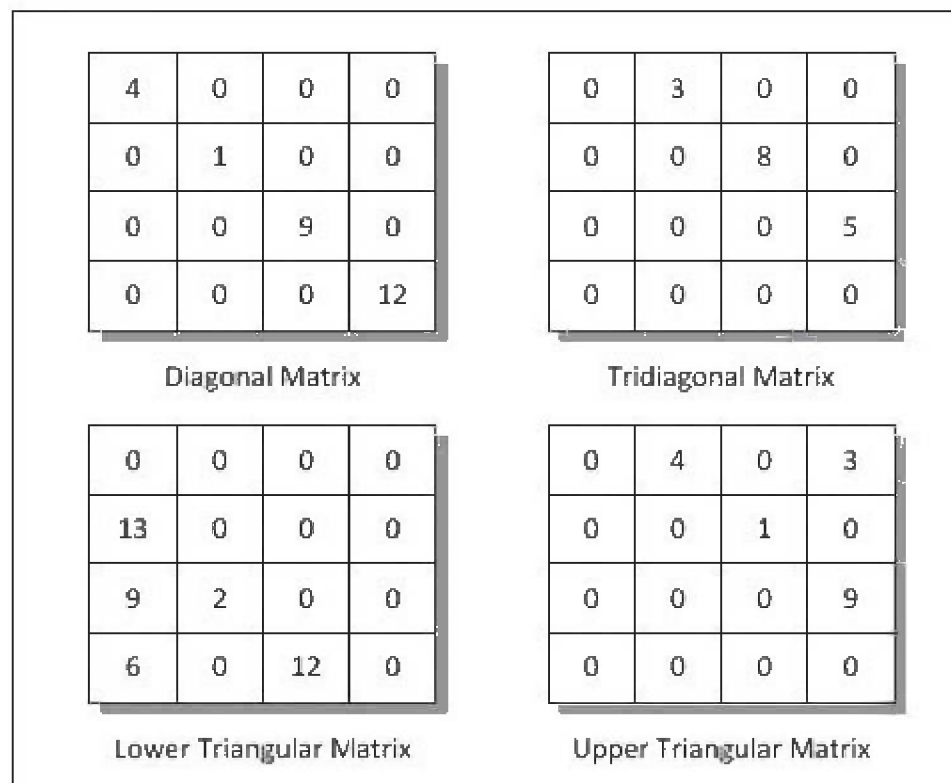
Figure 4-3. Different forms of Sparse matrices.
