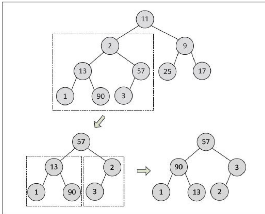
Figure 7-19. Multi-step heapify operation.
