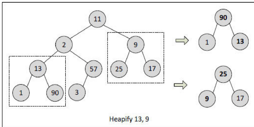
Figure 7-18. Heapify operation.
