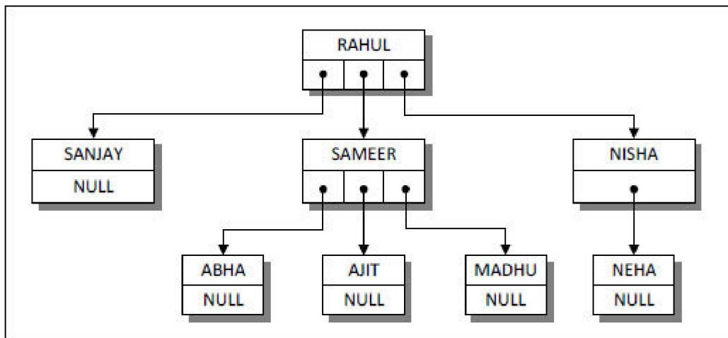
Figure 7-1. A tree
