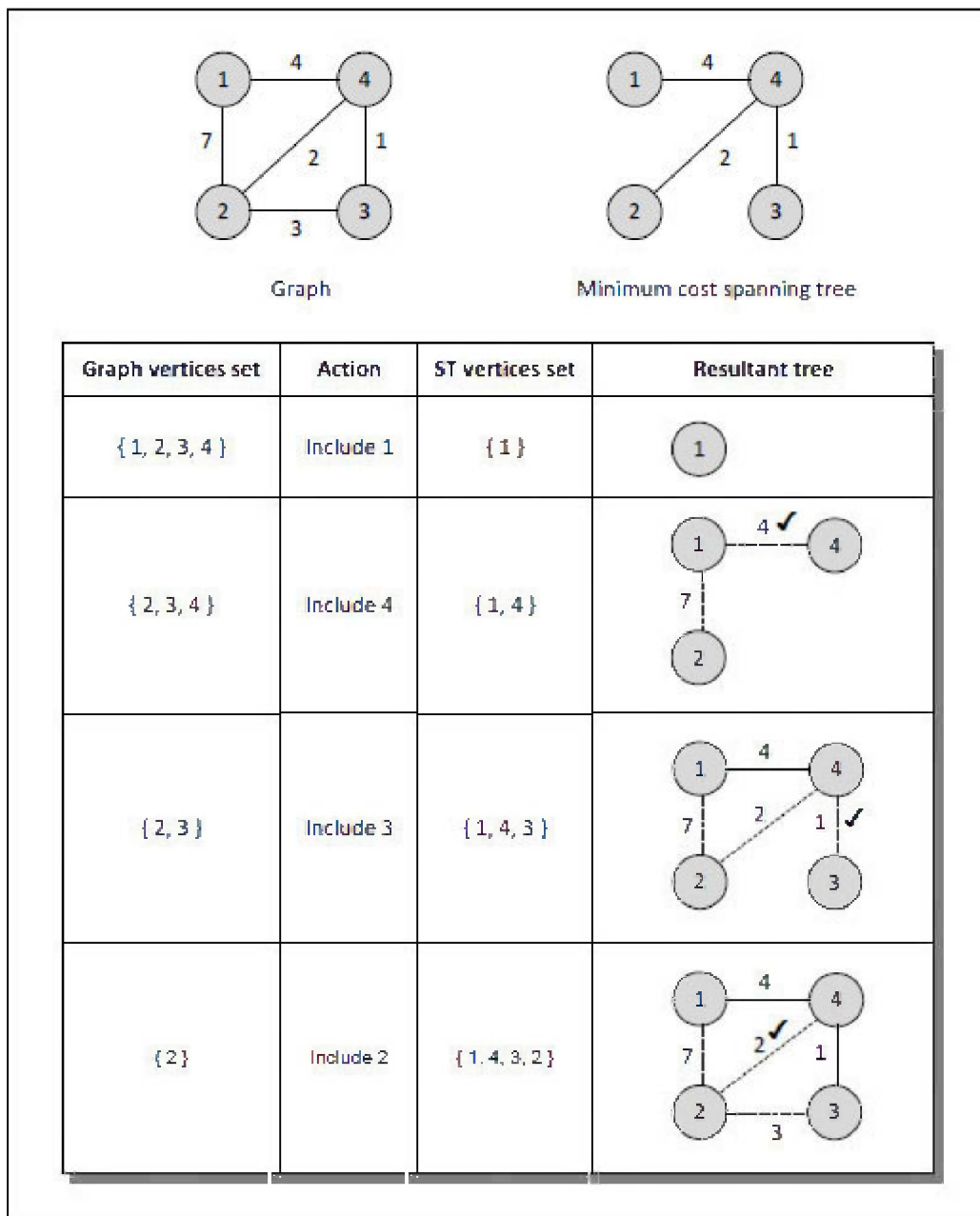
Figure 8-11. Minimum cost spanning tree using Prim's algorithm.
