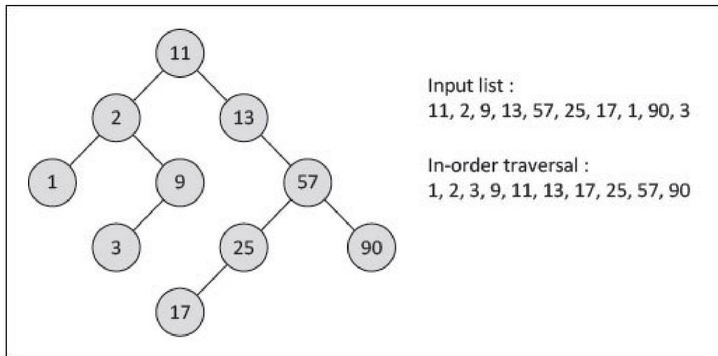
Figure 9-7. Binary Tree sort at work.
