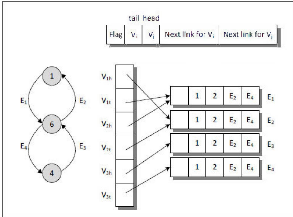
Figure 8-5. Adjacency multi-lists for directed graph.
