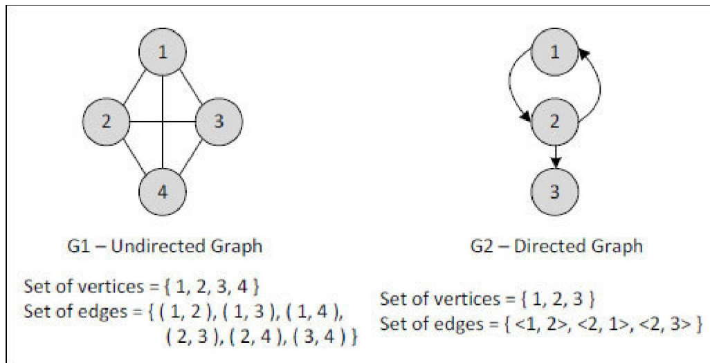
Figure 8-1. Directed and undirected
