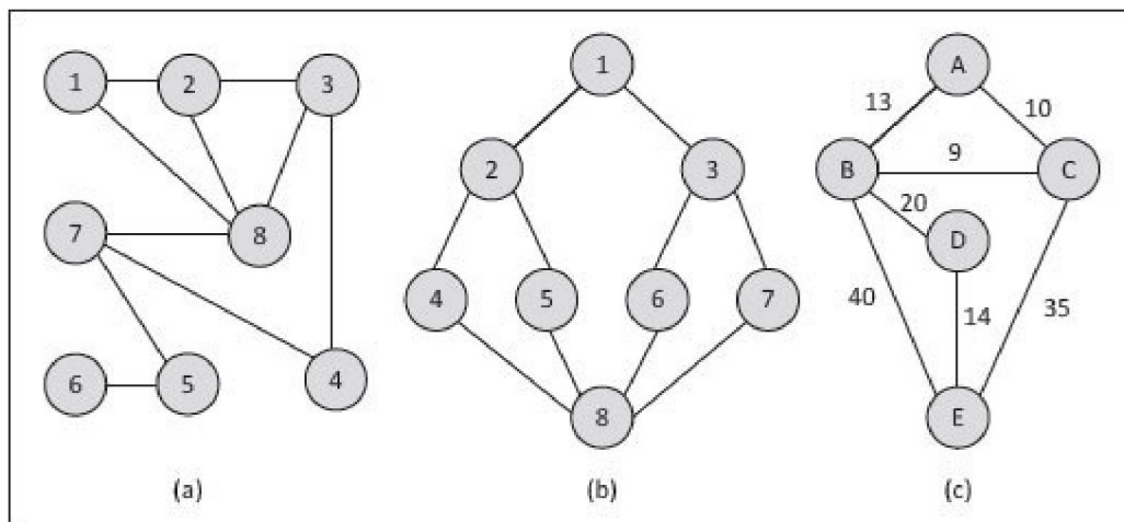
Figure 8-14. Graphs.
