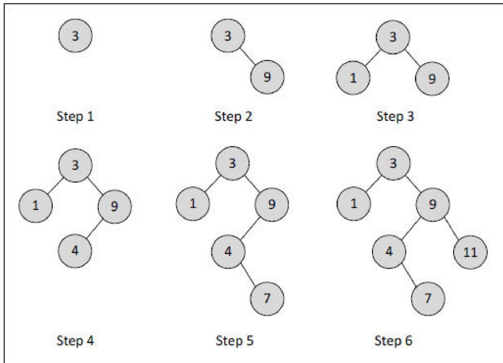
Figure 7-8. Creation of a Binary Search Tree.
