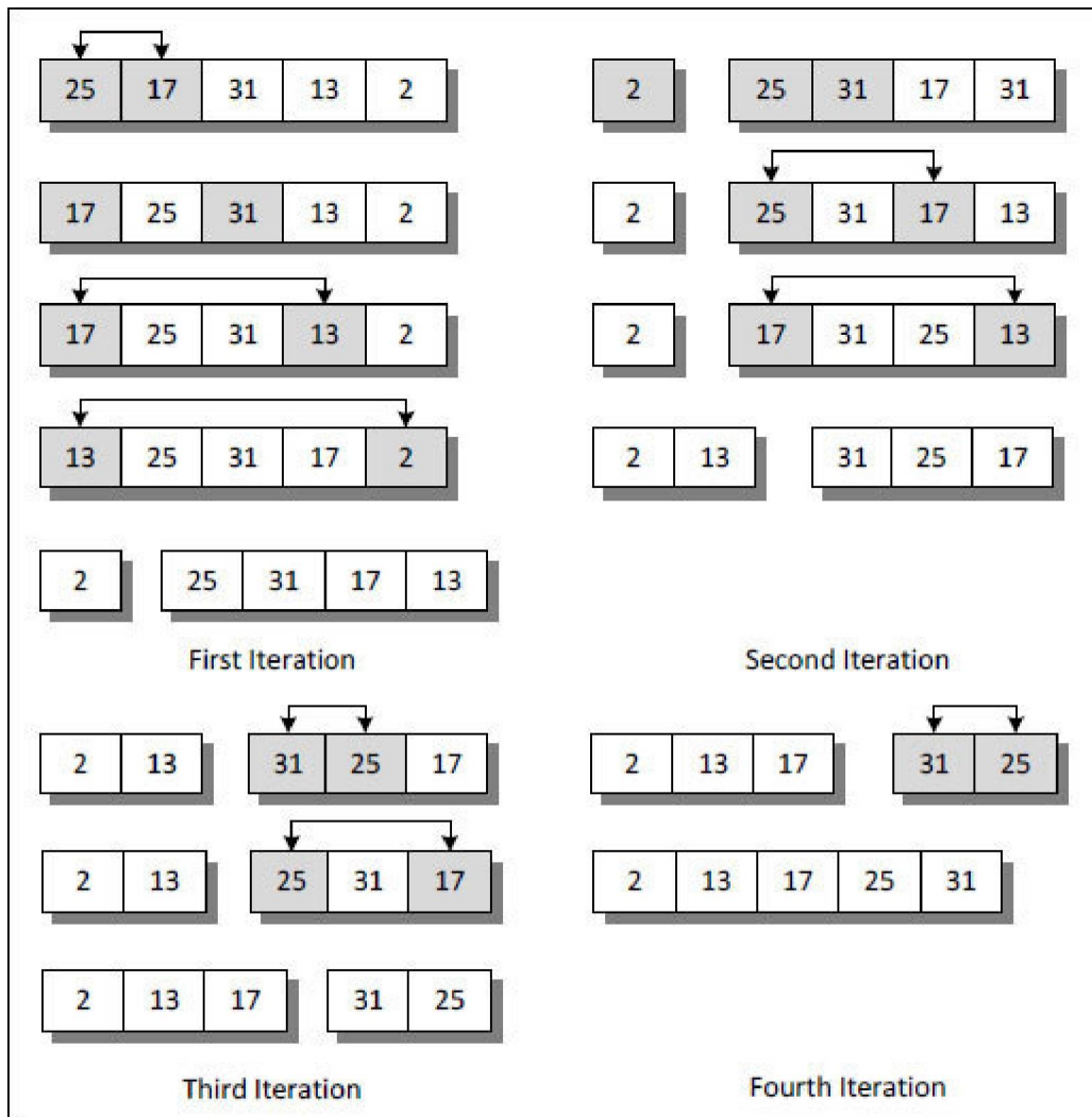
Figure 9-4. Selection sort at work.
