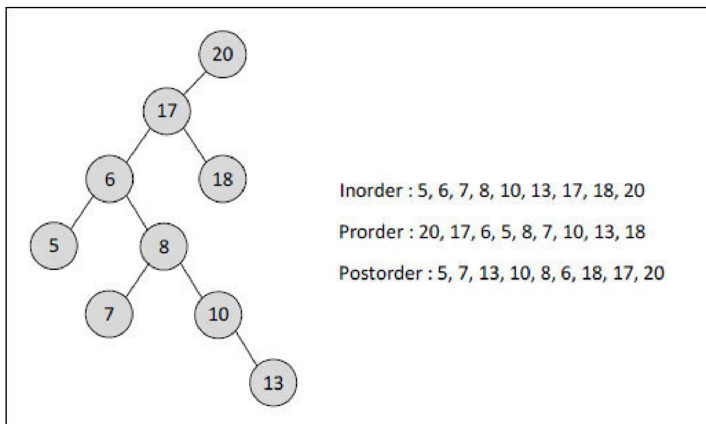
Figure 7-9. Traversals of binary tree.
