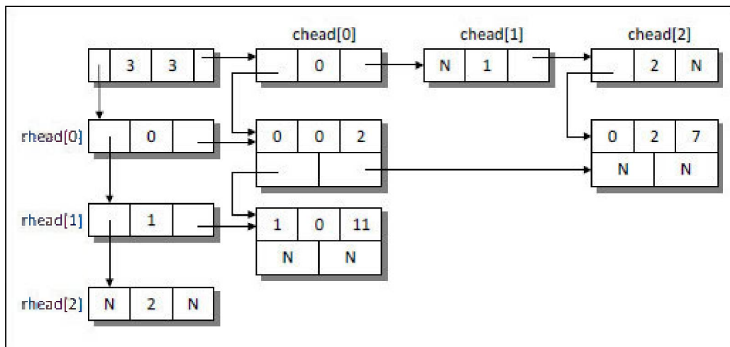
Figure 4-2. Linked Representation of a sparse matrix.
