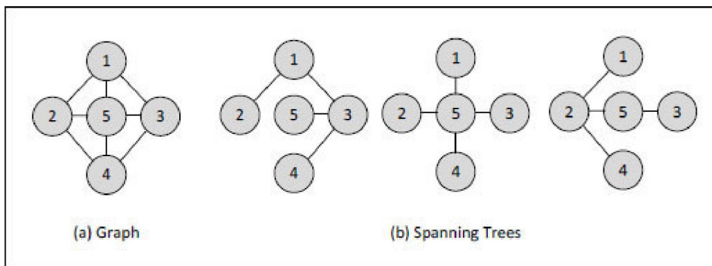
Figure 8-7. Graph and its spanning trees.
