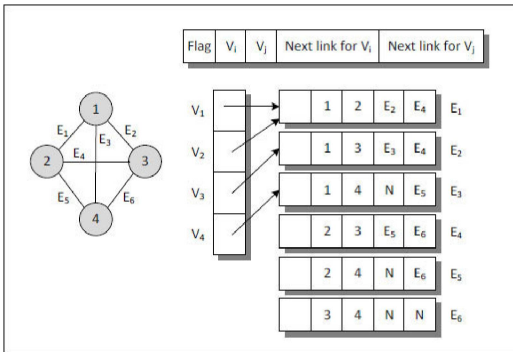
Figure 8-4. Adjacency multi-lists for undirected graph.
