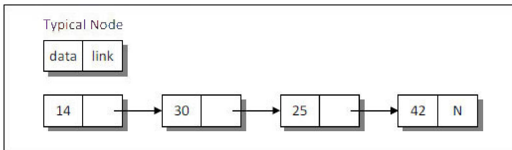
Figure 3-1. Linked list.
