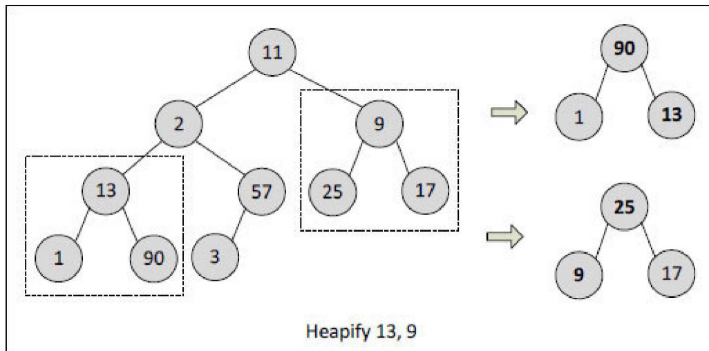
Figure 9-9. Heapify operation.
