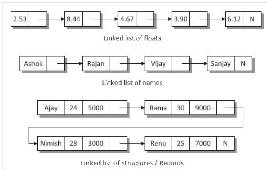
Figure 3-7. Different types of linked list.
