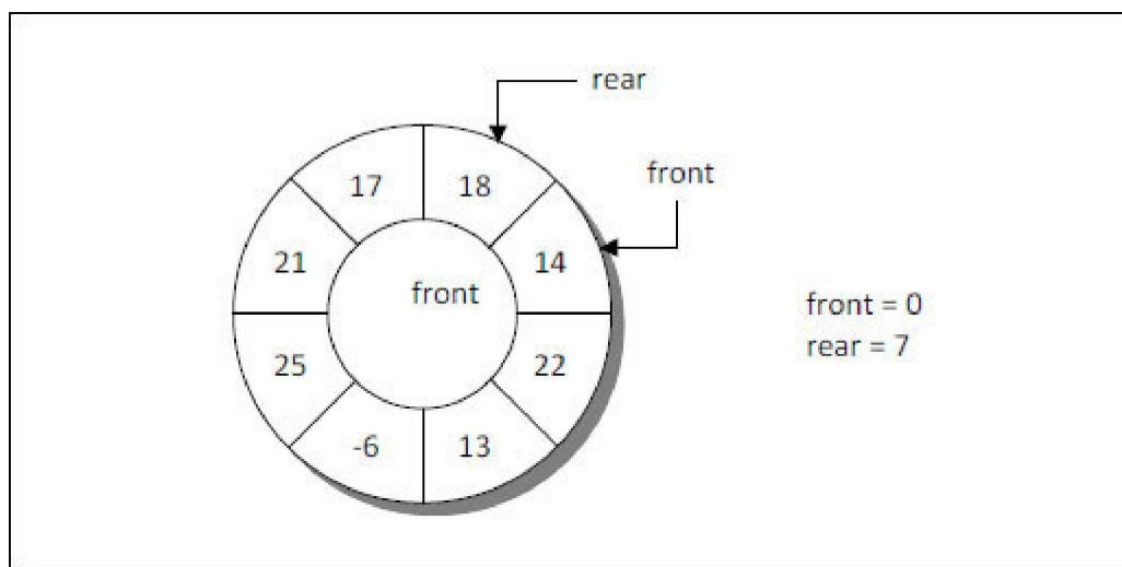
Figure 6-5. Circular queue after addition of 8 elements.
