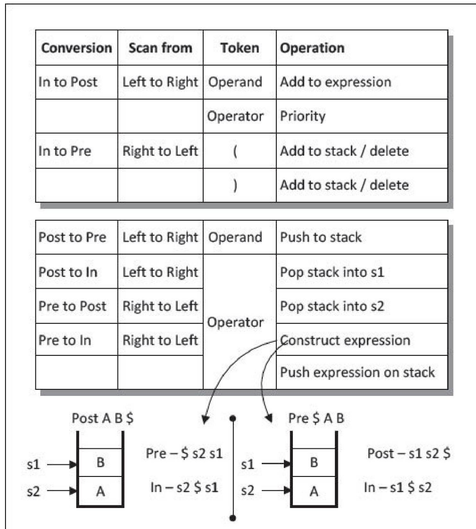
Figure 5-3. Summary of inter-conversion of expressions.
