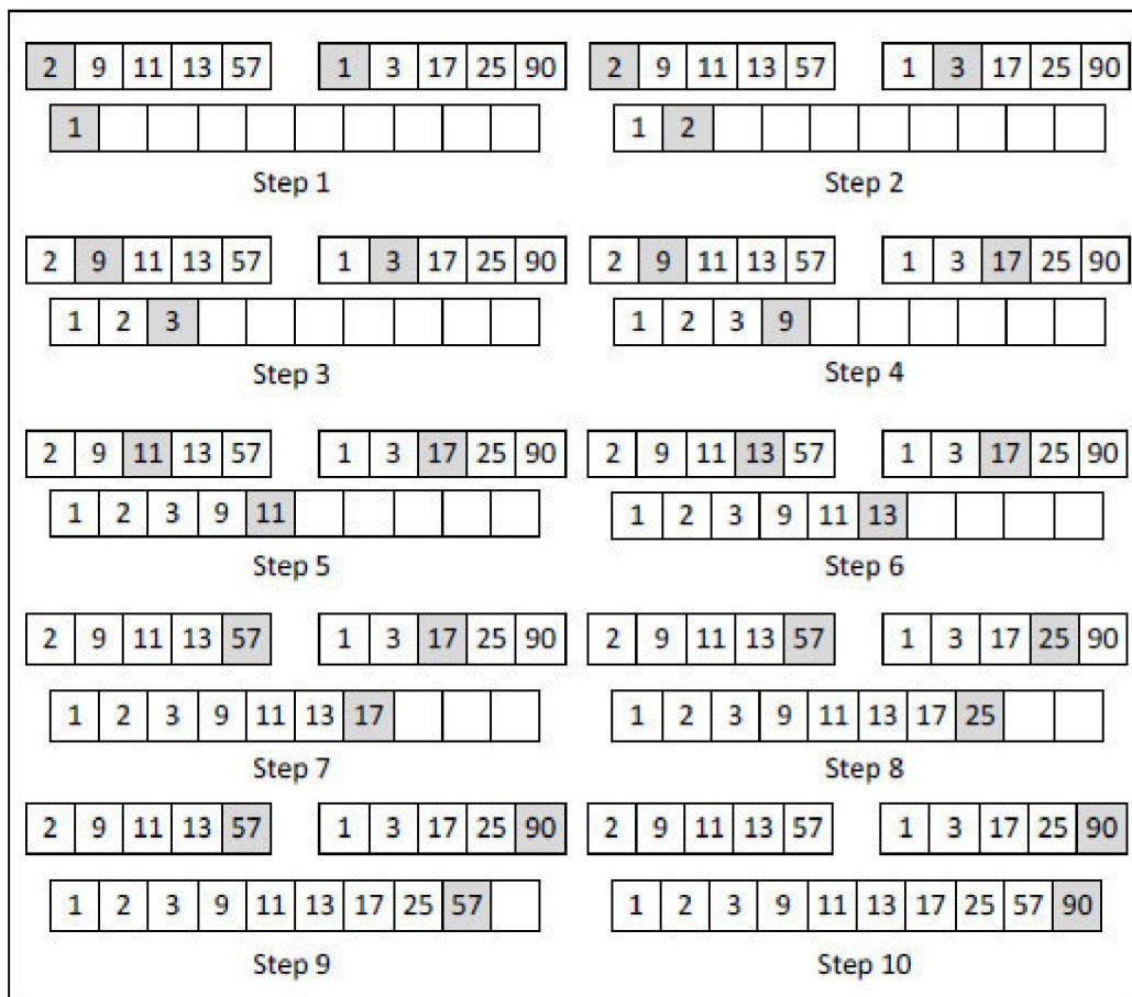
Figure 9-8. Merge sort at work.
