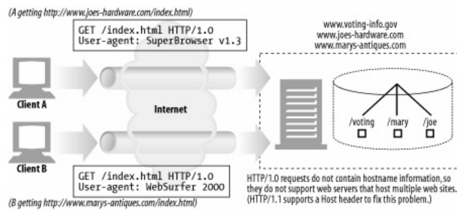
Figure 18-3. HTTP/1.0 server requests don't contain hostname information
