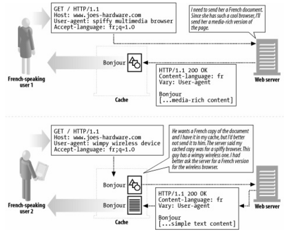
Figure 17-2. If servers vary on specific request headers, caches must match those request headers in addition to the regular content-negotiation headers before sending back cached responses
