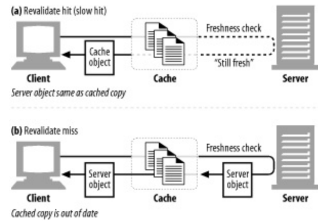
Figure 7-5. Successful revalidations are faster than cache misses; failed revalidations are nearly identical to misses
