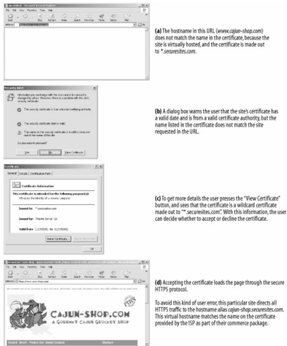
Figure 14-18. Certificate name mismatches bring up certificate error dialog boxes
