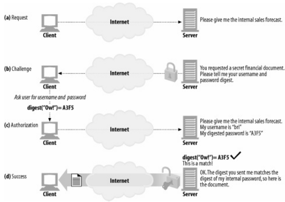
Figure 13-1. Using digests for password-obscured authentication
