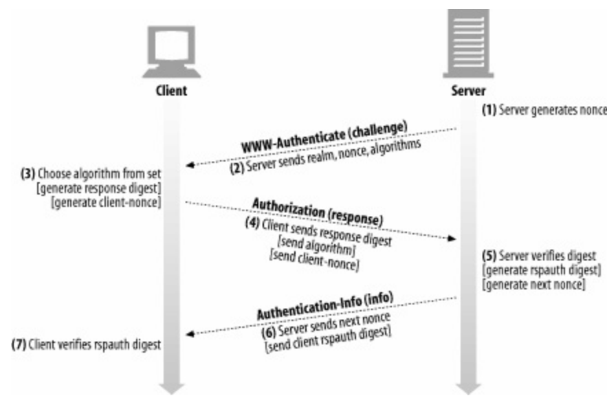
Figure 13-2. Digest authentication handshake
