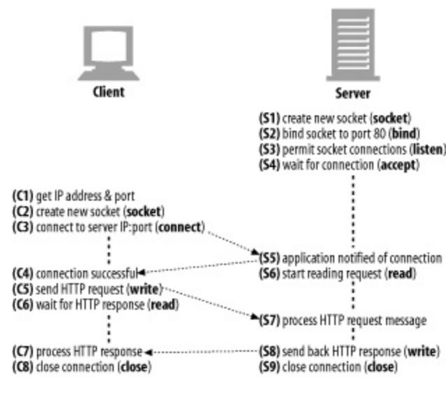
Figure 4-6. How TCP clients and servers communicate using the TCP sockets interface
