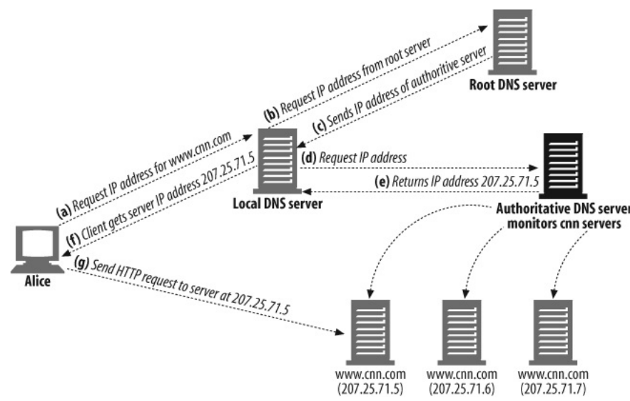
Figure 20-4. DNS request involving authoritative server
