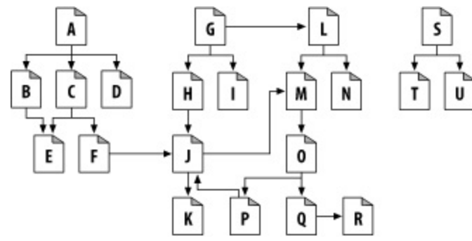
Figure 9-1. A root set is needed to reach all pages
