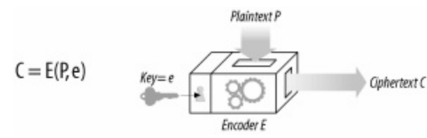
Figure 14-6. Plaintext is encoded with encoding key e , and decoded using decoding key d
