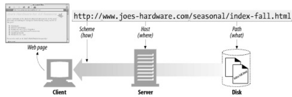
Figure 2-1. How URLs relate to browser, machine, server, and location on the server's filesystem
