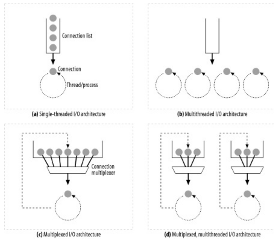
Figure 5-7. Web server input/output architectures
