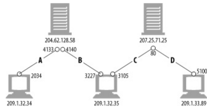
Figure 4-5. Four distinct TCP connections
