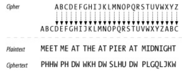
Figure 14-4. Rotate-by-3 cipher example
