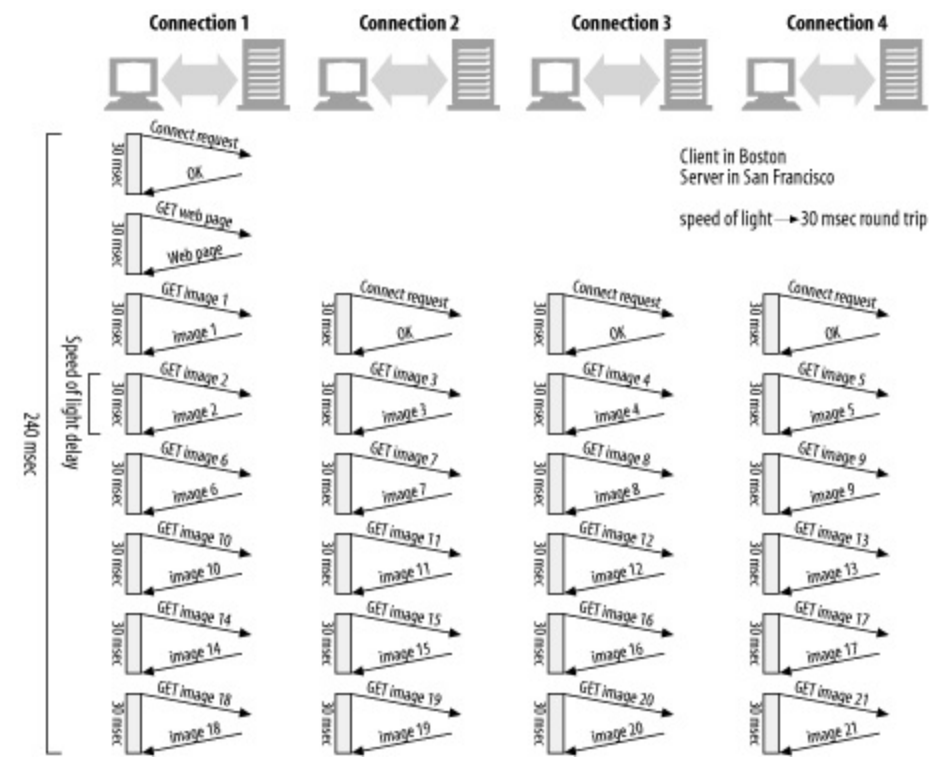
Figure 7-3. Speed of light can cause significant delays, even with parallel, keep-alive connections
