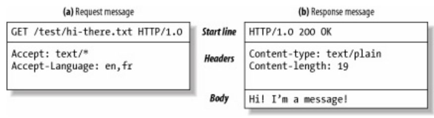
Figure 1-7. HTTP messages have a simple, line-oriented text structure
