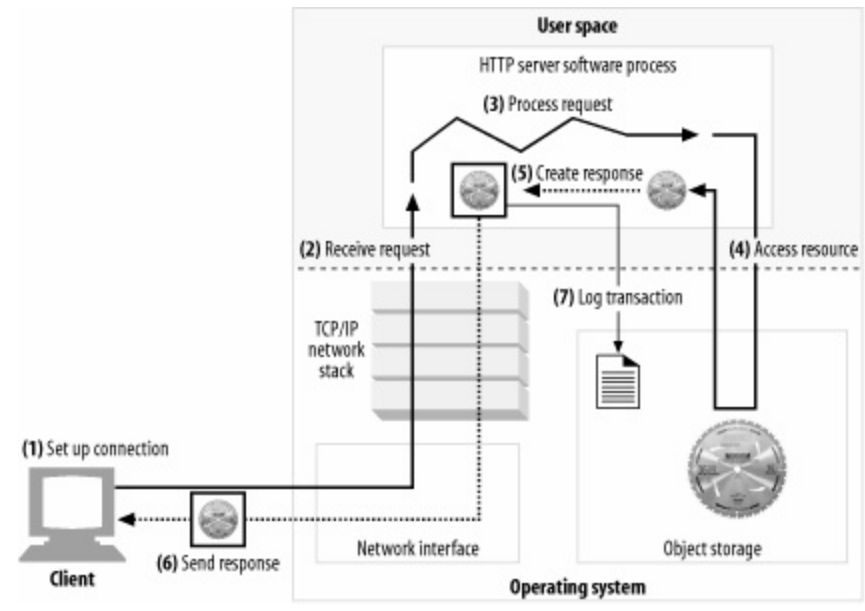
Figure 5-3. Steps of a basic web server request
