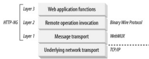
Figure 10-1. HTTP-NG separates functions into layers
