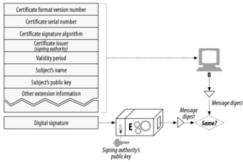
Figure 14-12. Verifying that a signature is real
