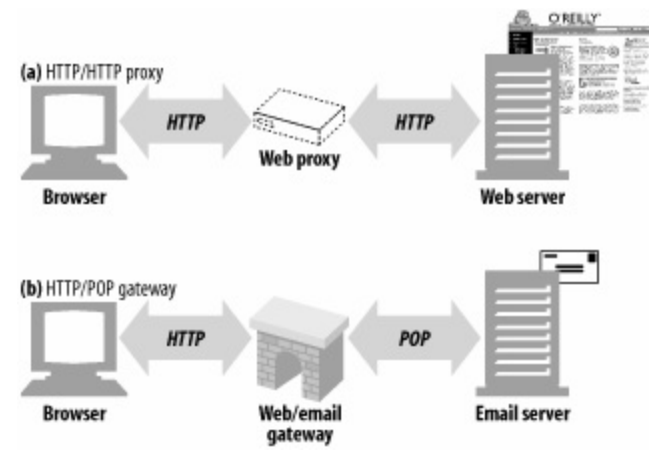
Figure 6-2. Proxies speak the same protocol; gateways tie together different protocols
