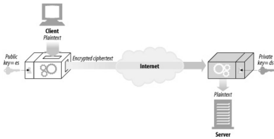
Figure 14-8. Public-key cryptography is asymmetric, using different keys for encoding and decoding
