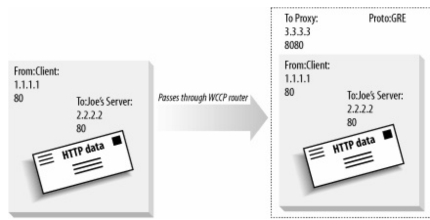
Figure 20-12. How a WCCP router changes an HTTP packet's destination IP address
