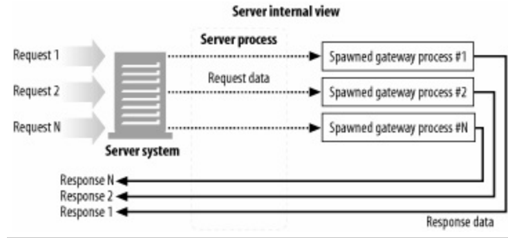
Figure 8-9. Server gateway application mechanics
