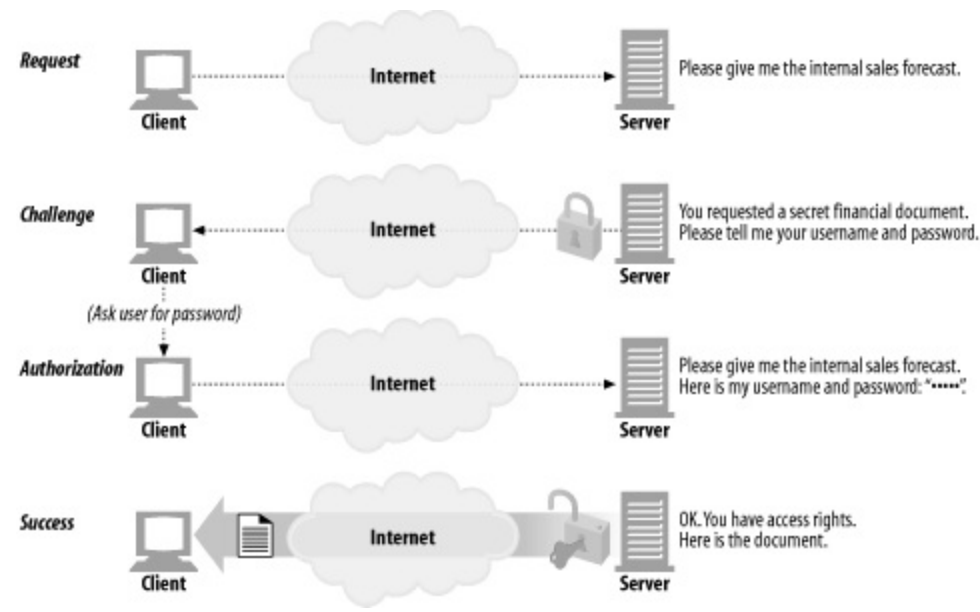
Figure 12-1. Simplified challenge/response authentication
