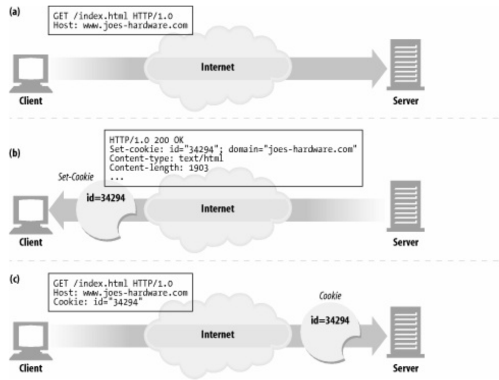
Figure 11-3. Slapping a cookie onto a user
