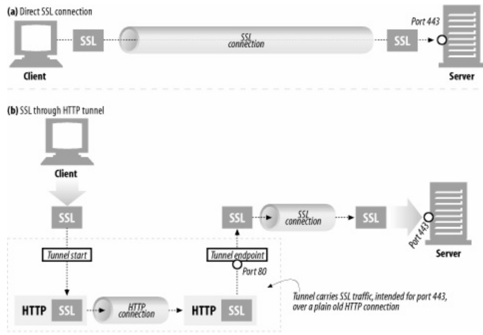
Figure 8-12. Direct SSL connection vs. tunnelled SSL connection
