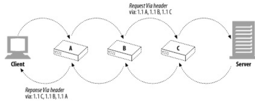
Figure 6-21. The response Via is usually the reverse of the request Via
