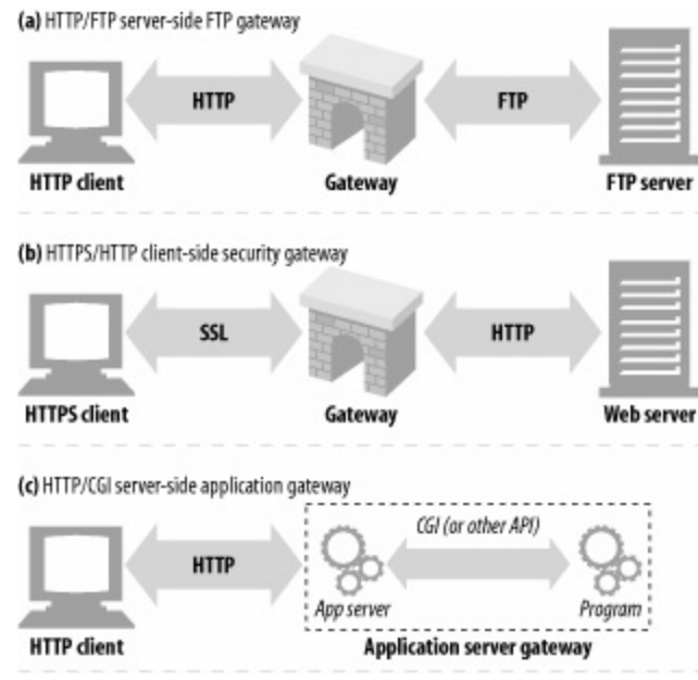
Figure 8-2. Three web gateway examples
