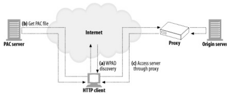
Figure 20-11. WPAD determines the PAC URL, which determines the proxy server
