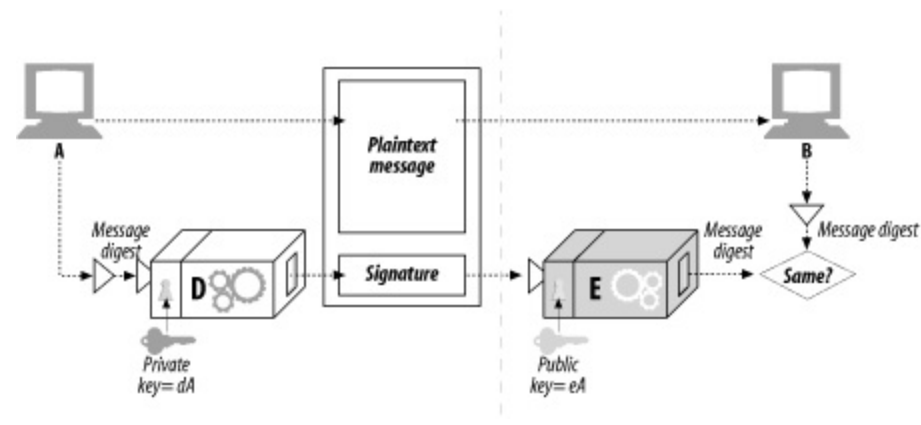
Figure 14-10. Unencrypted digital signature
