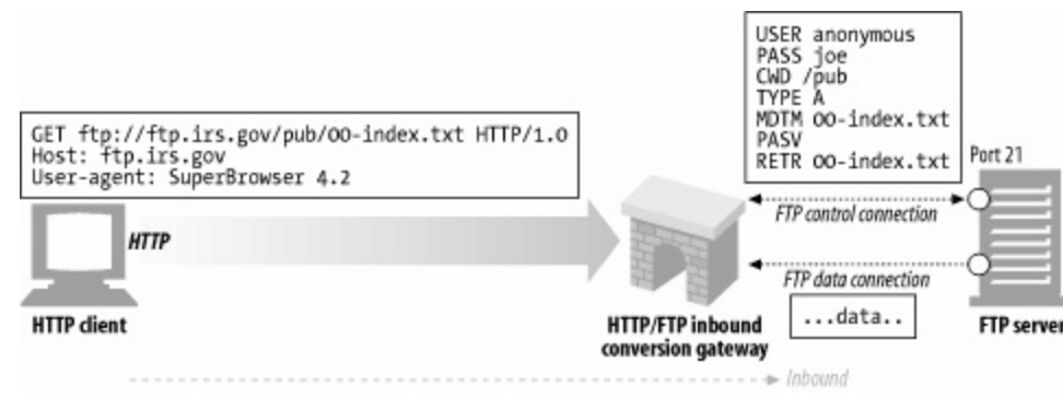
Figure 8-5. The HTTP/FTP gateway translates HTTP request into FTP requests
