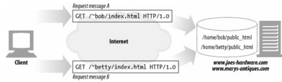
Figure 5-10. Different docroots for different users
