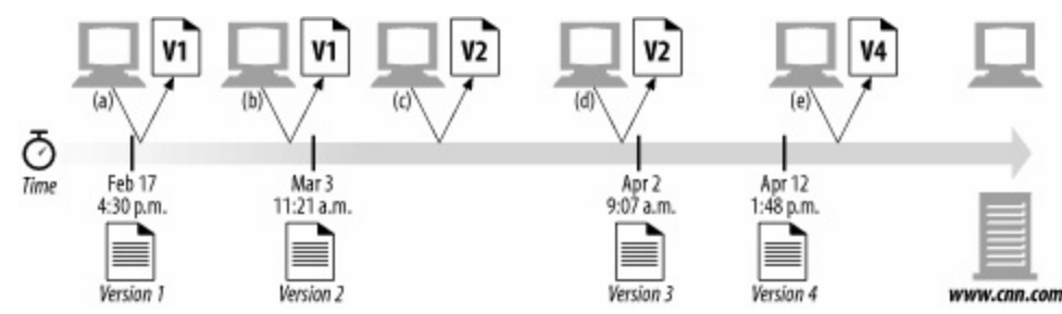
Figure 15-8. Instances are “snapshots” of a resource in time
