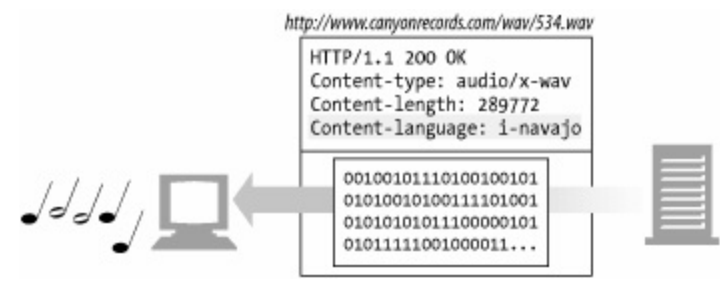
Figure 16-8. Content-Language header marks a “Rain Song” audio clip for Navajo speakers
