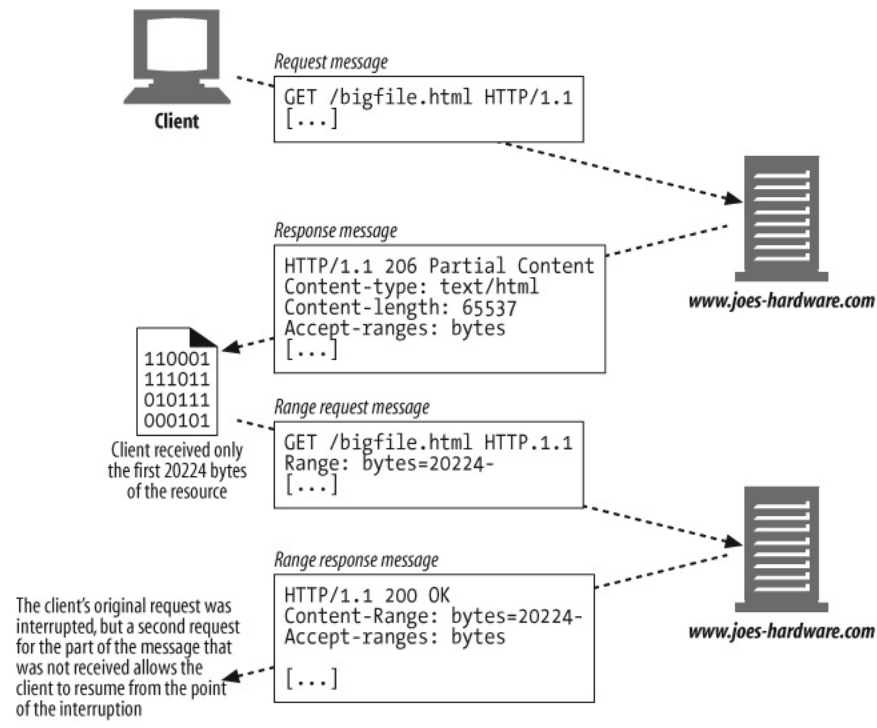
Figure 15-9. Entity range request example
