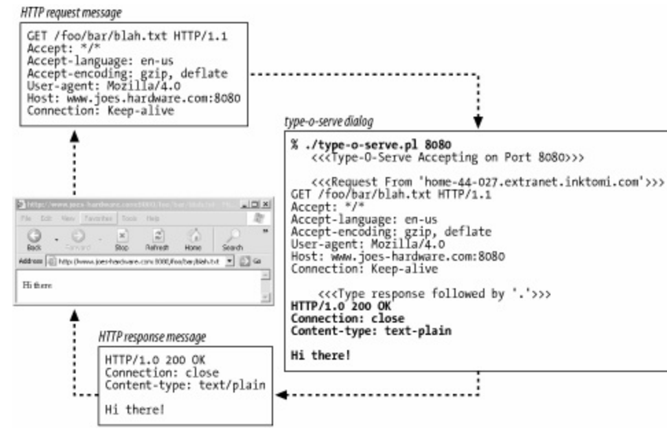
Figure 5-2. The type-o-serve utility lets you type in server responses to send back to clients
