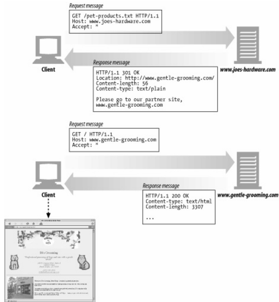
Figure 3-14. Redirected request to new location
