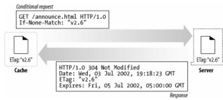
Figure 7-15. If-None-Match revalidates because entity tag still matches
