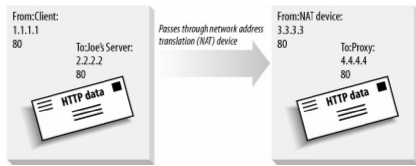
Figure 20-9. Full NAT of a TCP/IP datagram
