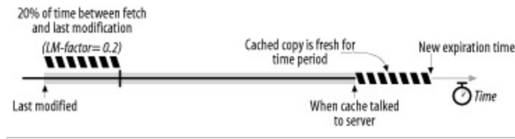
Figure 7-16. Computing a freshness period using the LM-Factor algorithm
