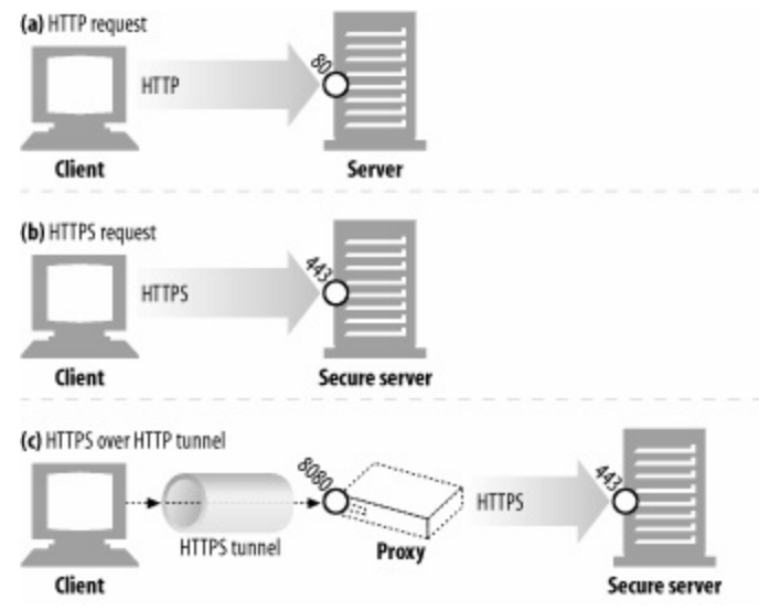
Figure 14-14. HTTP and HTTPS port numbers
