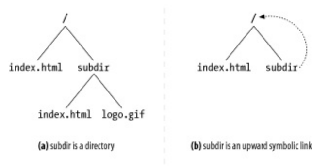
Figure 9-3. Symbolic link cycles
