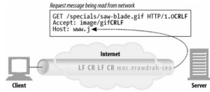
Figure 5-5. Reading a request message from a connection
