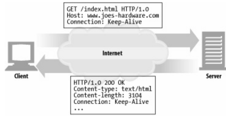
Figure 4-14. HTTP/1.0 keep-alive transaction header handshake
