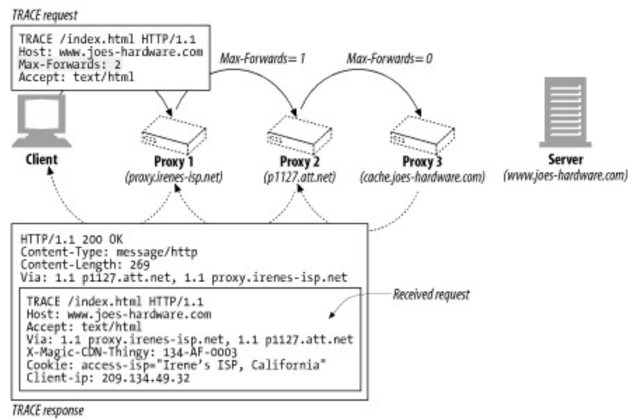
Figure 6-24. You can limit the forwarding hop count with the Max-Forwards header field
