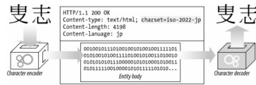
Figure 16-7. Character encoding scheme encodes character codes into bits and back again
