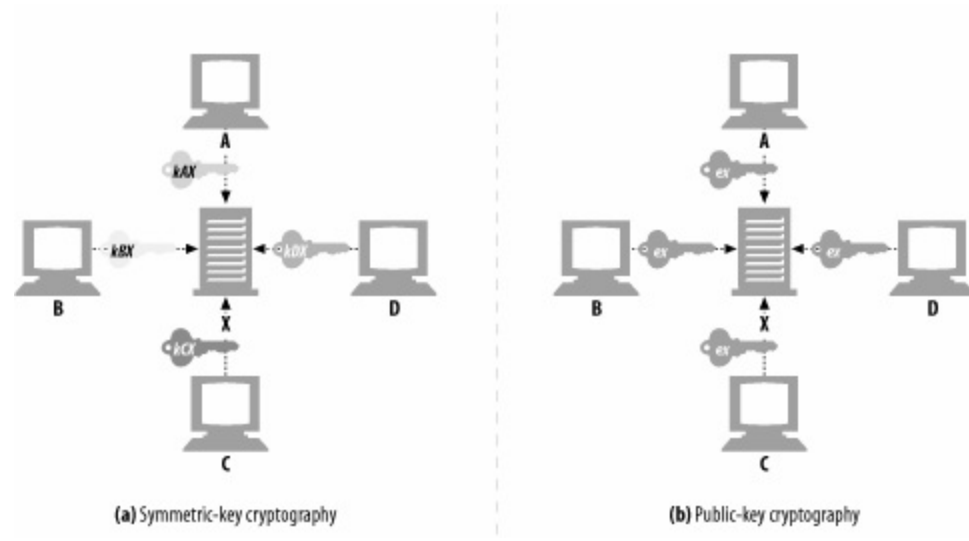
Figure 14-9. Public-key cryptography assigns a single, public encoding key to each host
