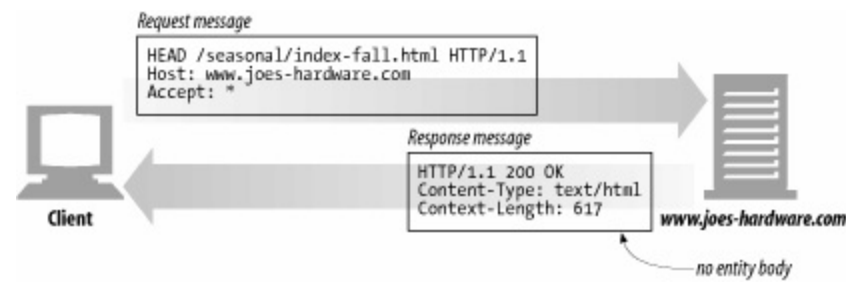
Figure 3-8. HEAD example
