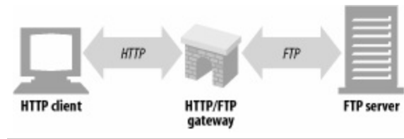
Figure 1-13. HTTP/FTP gateway
