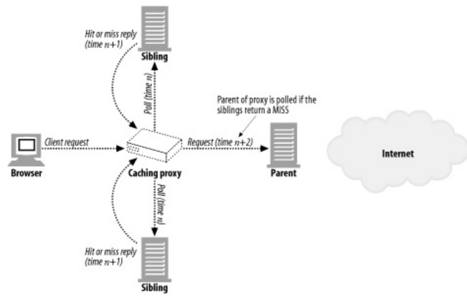
Figure 20-13. ICP queries
