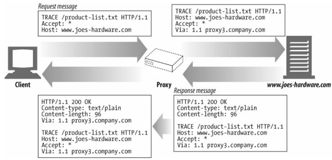
Figure 3-11. TRACE example
