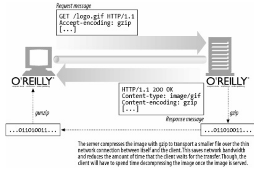
Figure 15-4. Content encoding
