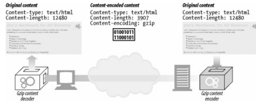
Figure 15-3. Content-encoding example
