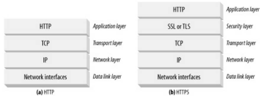
Figure 14-13. HTTP transport-level security
