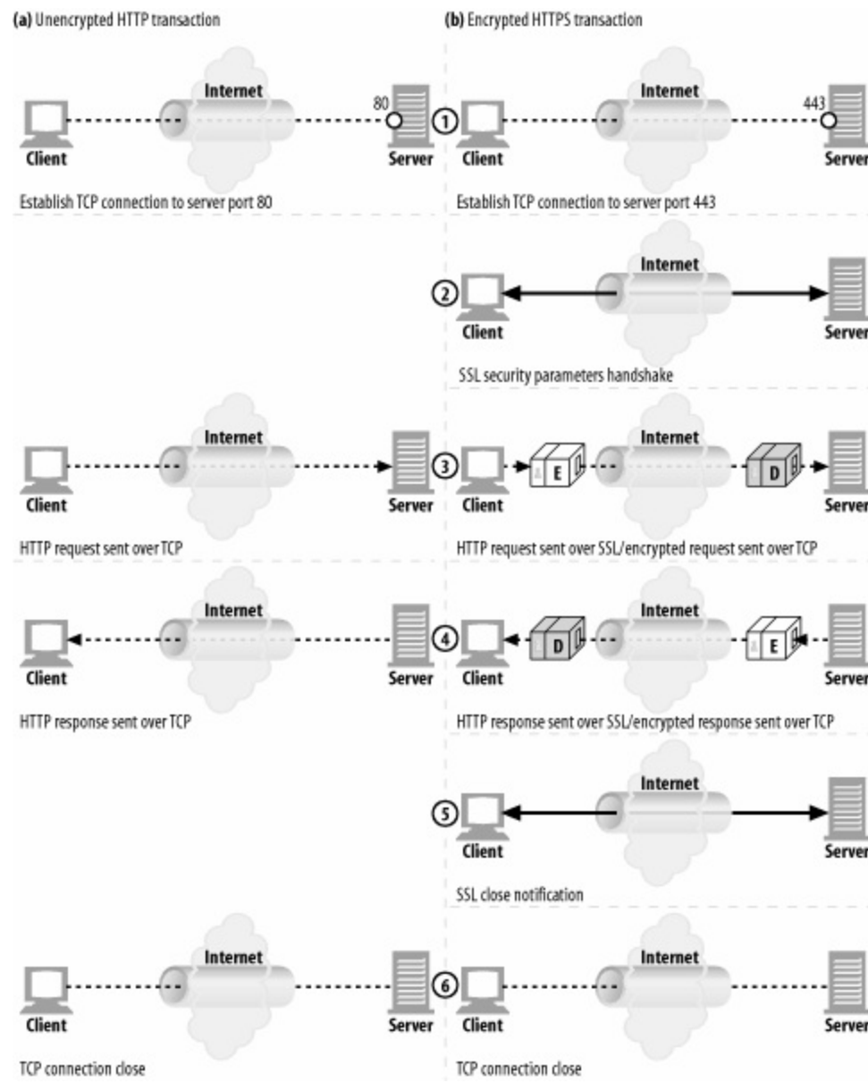
Figure 14-15. HTTP and HTTPS transactions
