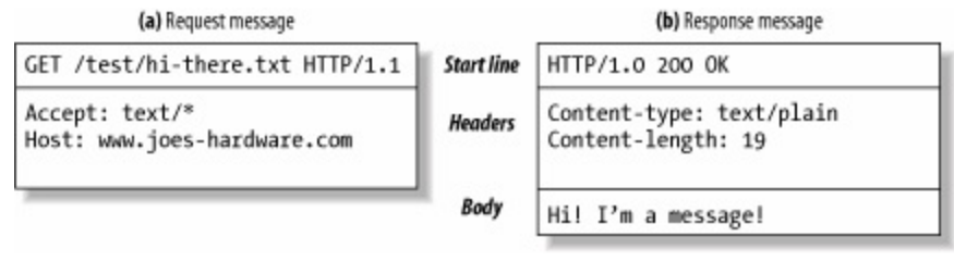
Figure 3-5. Example request and response messages
