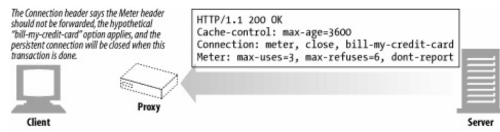
Figure 4-9. The Connection header allows the sender to specify connection-specific options
