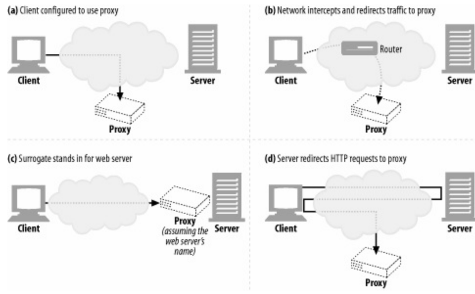
Figure 6-14. There are many techniques to direct web requests to proxies
