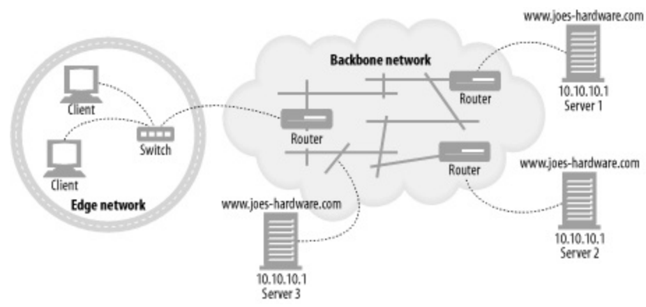
Figure 20-5. Distributed anycast addressing
