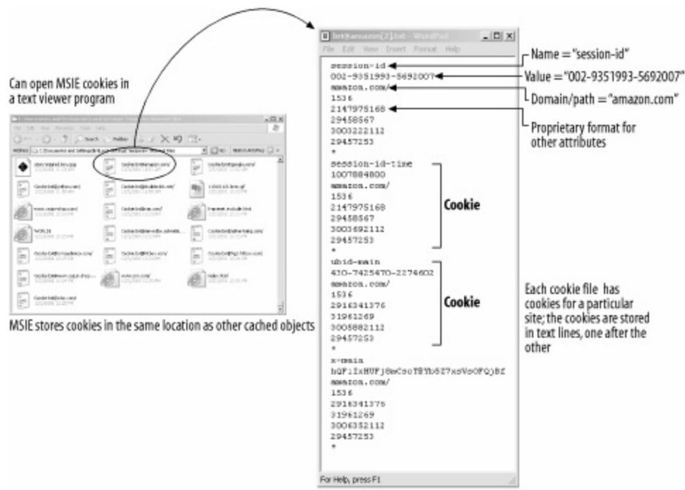
Figure 11-4. Internet Explorer cookies are stored in individual text files in the cache directory
