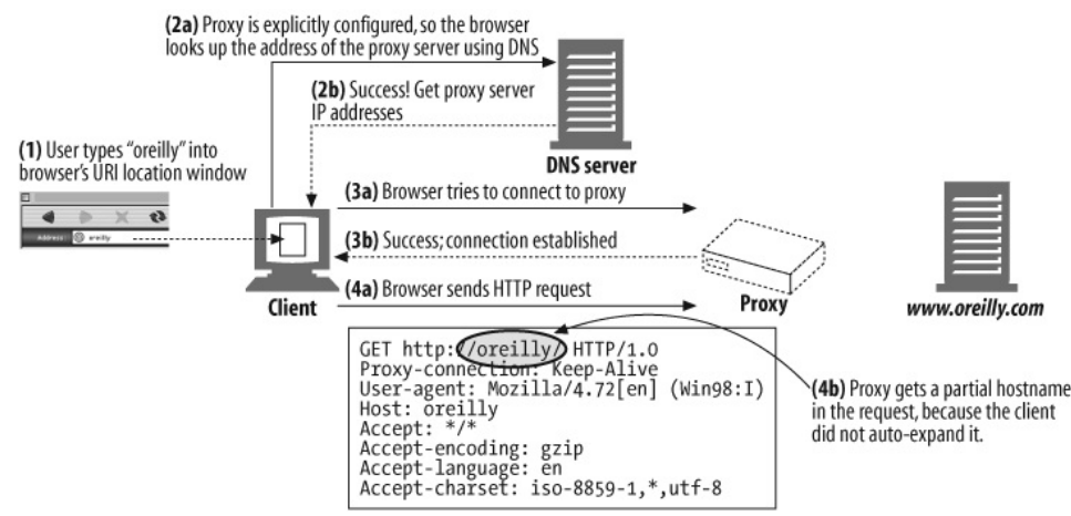
Figure 6-17. Browser does not auto-expand partial hostnames when there is an explicit proxy
