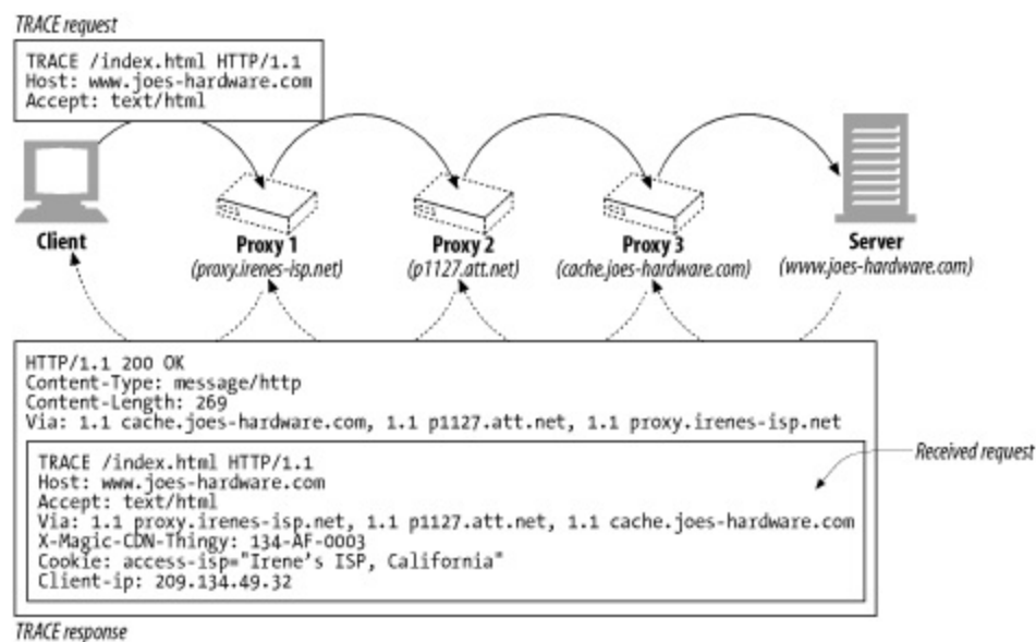
Figure 6-23. TRACE response reflects back the received request message
