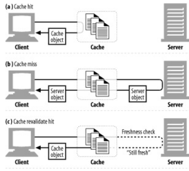
Figure 7-4. Cache hits, misses, and revalidations
