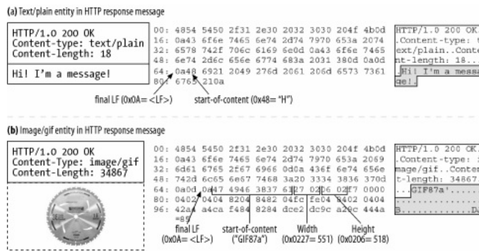
Figure 15-2. Hex dumps of real message content (raw message content follows blank CRLF)
