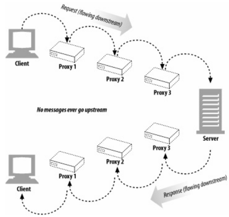
Figure 3-2. All messages flow downstream
