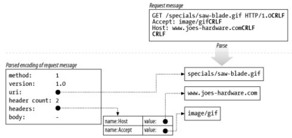
Figure 5-6. Parsing a request message into a convenient internal representation
