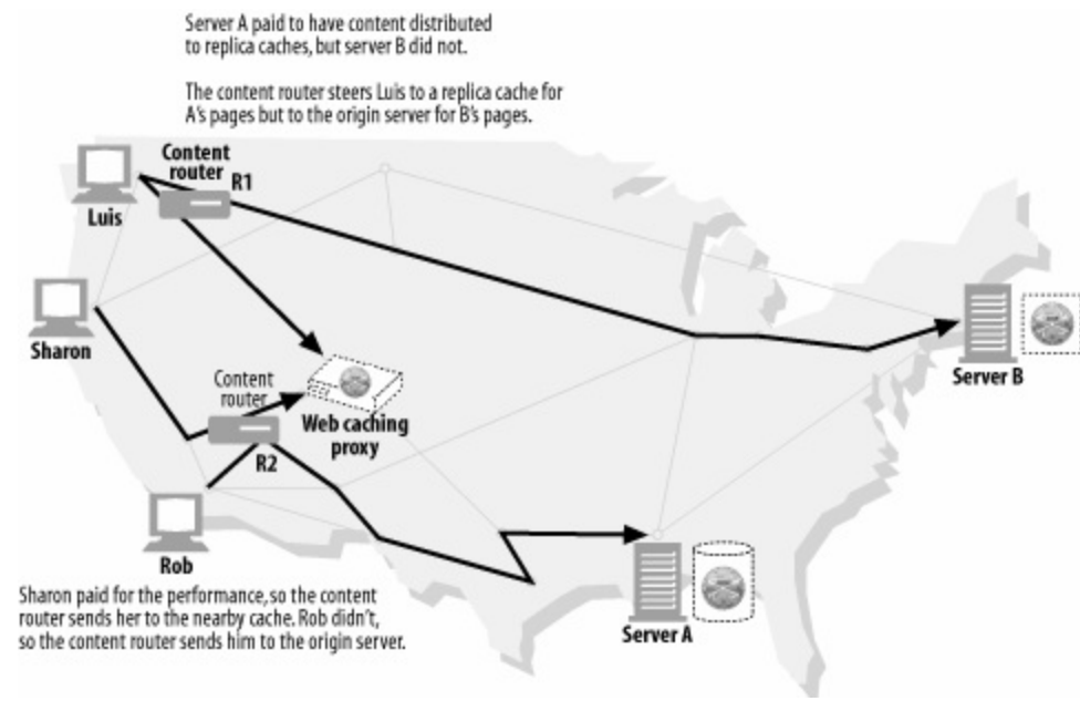
Figure 6-8. Proxy application example: content routing
