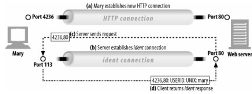
Figure 5-4. Using the ident protocol to determine HTTP client username
