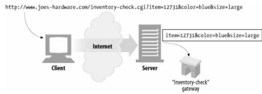
Figure 2-2. The URL query component is sent along to the gateway application
