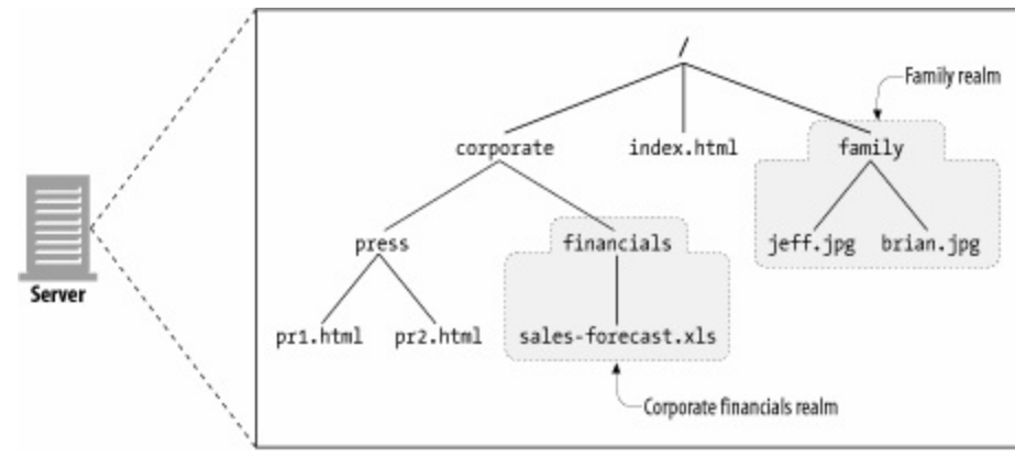
Figure 12-3. Security realms in a web server
