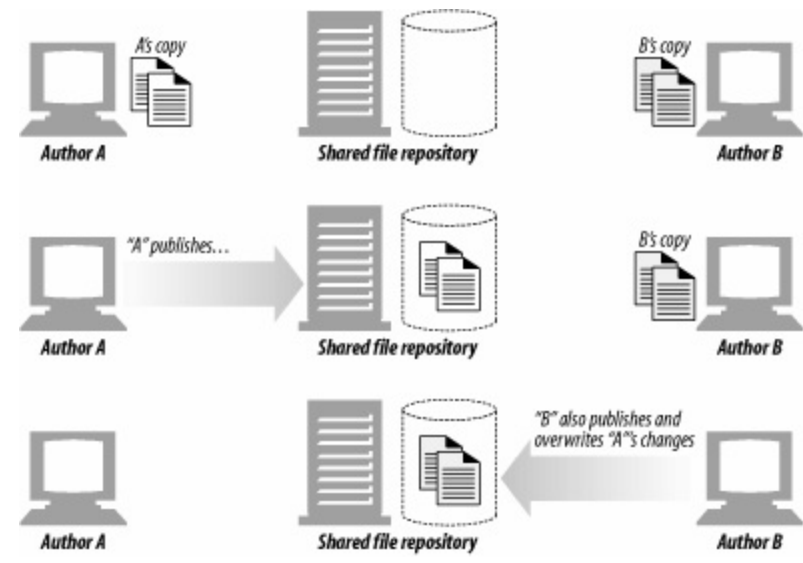
Figure 19-3. Lost update problem
