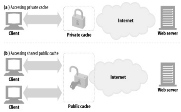
Figure 7-7. Public and private caches
