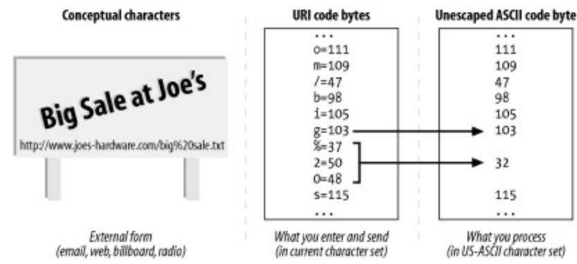
Figure 16-10. URI characters are transported as escaped code bytes but processed unescaped
