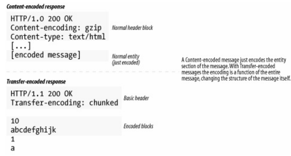
Figure 15-5. Content encodings versus transfer encodings
