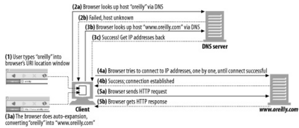
Figure 6-16. Browser auto-expands partial hostnames when no explicit proxy is present
