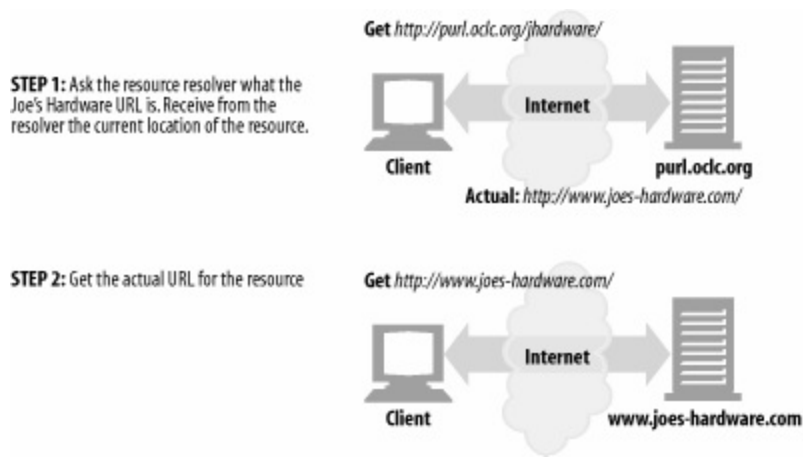
Figure 2-6. PURLs use a resource locator server to name the current location of a resource
