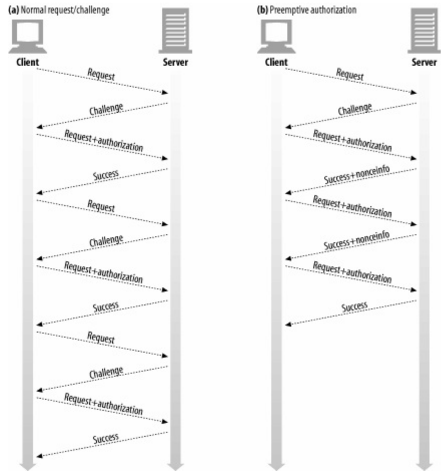
Figure 13-4. Preemptive authorization reduces message count
