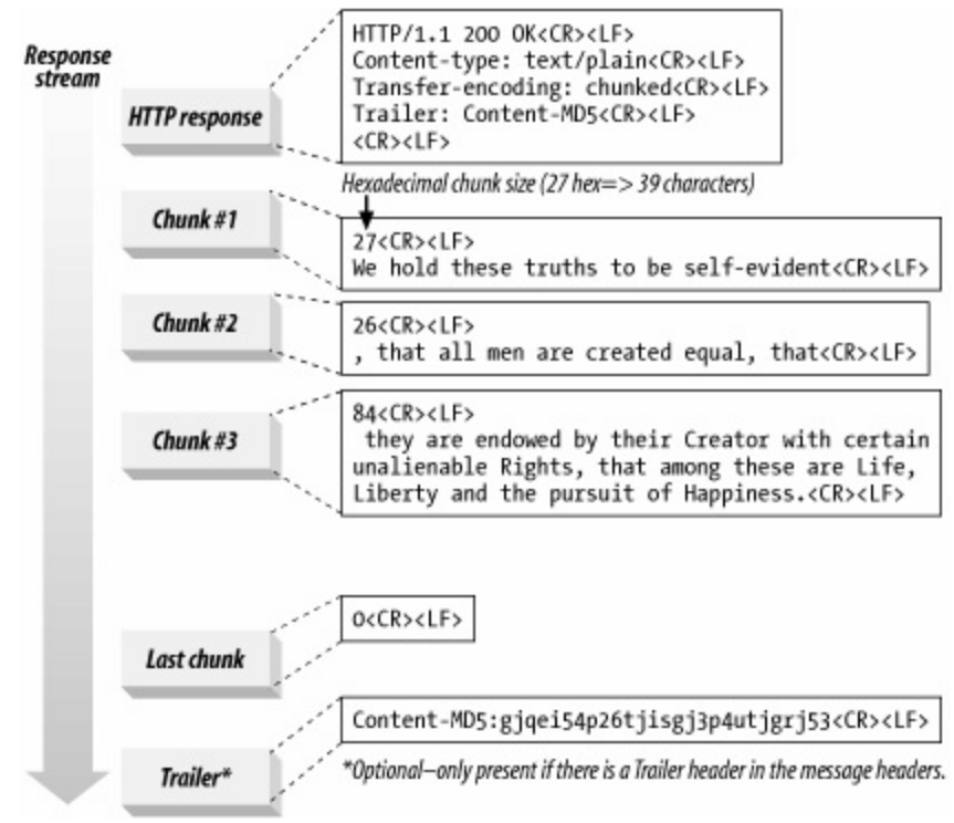
Figure 15-6. Anatomy of a chunked message
