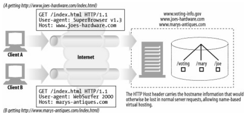
Figure 18-5. Host headers distinguish virtual host requests
