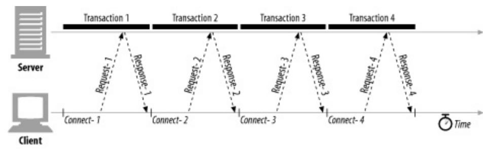
Figure 4-10. Four transactions (serial)
