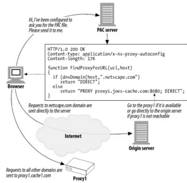
Figure 20-10. Proxy auto-configuration
