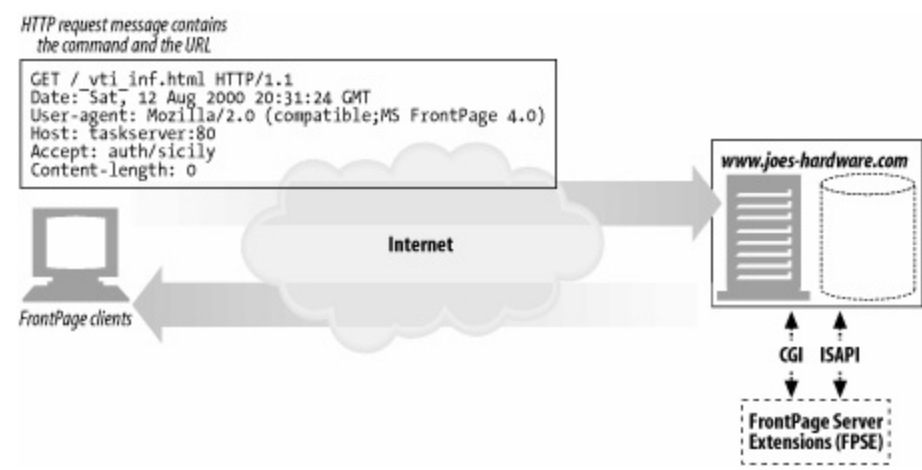
Figure 19-2. Initial request
