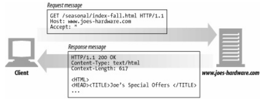
Figure 3-7. GET example
