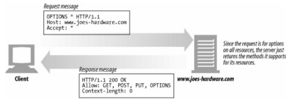
Figure 3-12. OPTIONS example
