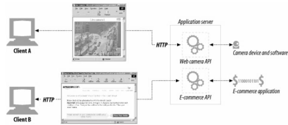
Figure 8-8. An application server connects HTTP clients to arbitrary backend applications
