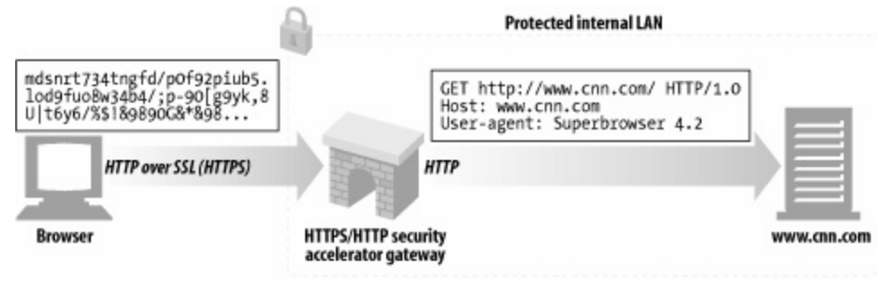
Figure 8-7. HTTPS/HTTP security accelerator gateway
