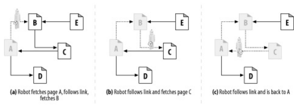
Figure 9-2. Crawling over a web of hyperlinks
