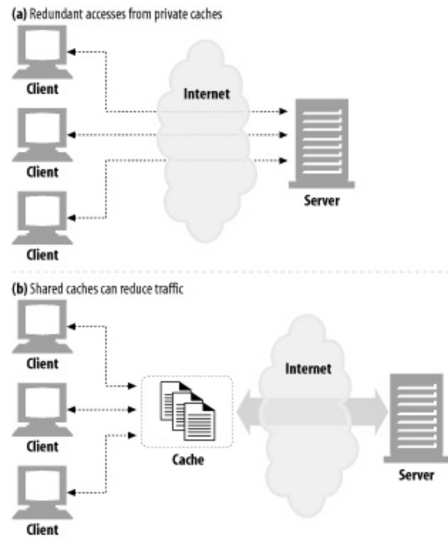
Figure 7-8. Shared, public caches can decrease network traffic
