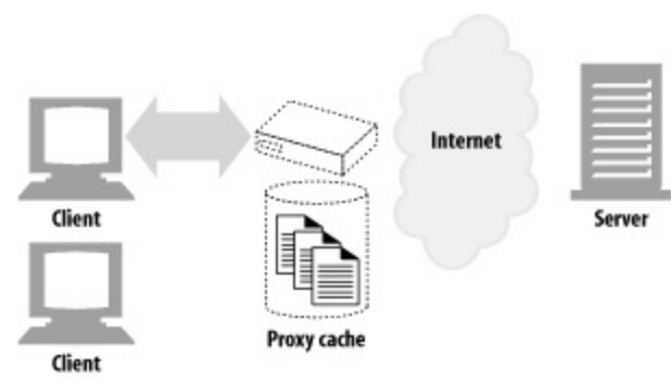
Figure 1-12. Caching proxies keep local copies of popular documents to improve performance
