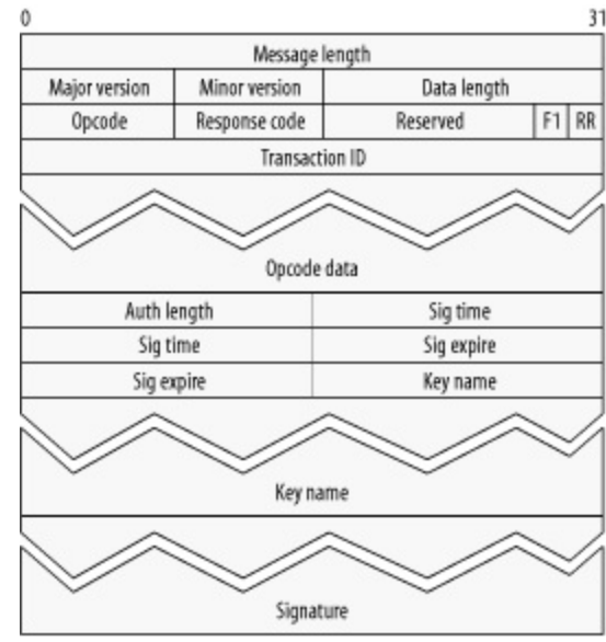
Figure 20-15. HTCP message format
