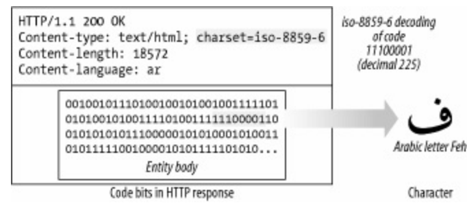
Figure 16-1. The charset parameter tells the client how to go from bits to characters
