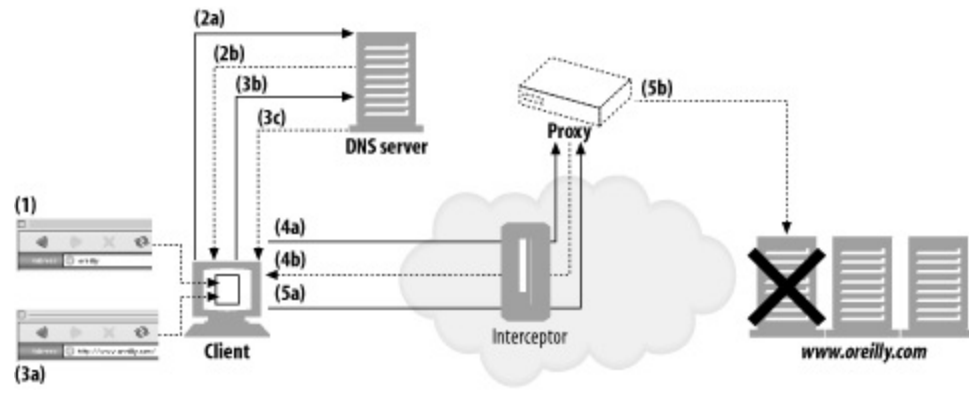
Figure 6-18. Browser doesn't detect dead server IP addresses when using intercepting proxies
