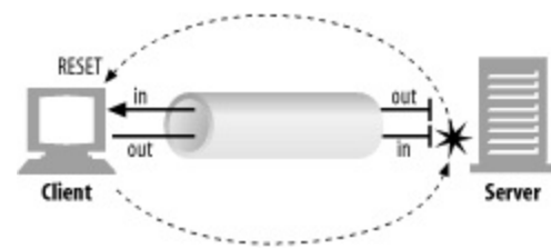
Figure 4-21. Data arriving at closed connection generates "connection reset by peer" error
