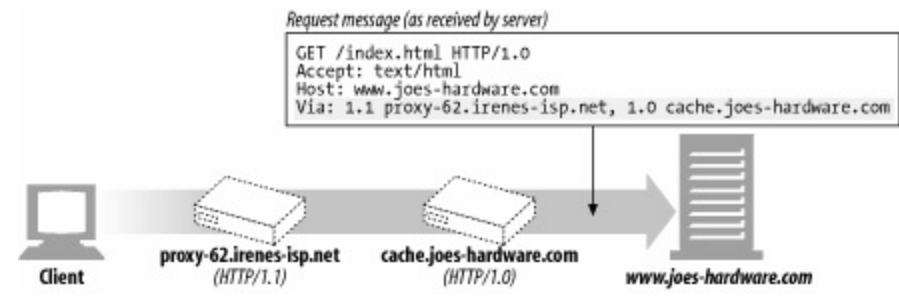
Figure 6-20. Via header example
