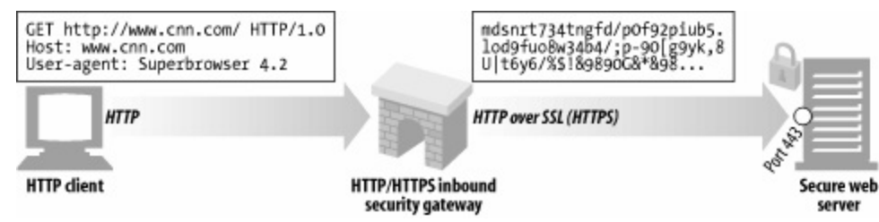
Figure 8-6. Inbound HTTP/HTTPS security gateway
