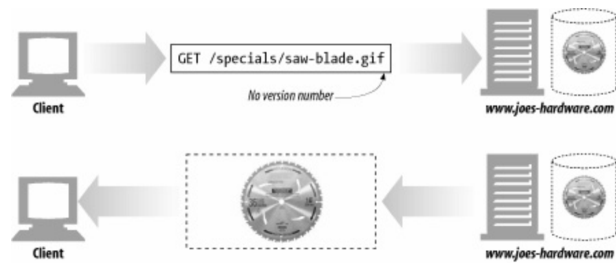
Figure 3-6. HTTP/0.9 transaction
