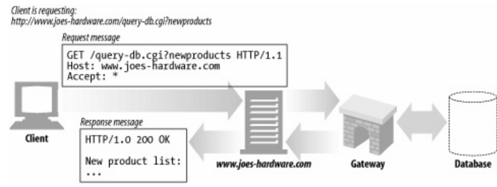
Figure 8-1. Gateway magic
