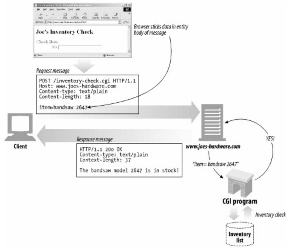
Figure 3-10. POST example
