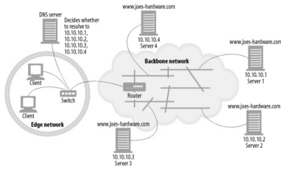
Figure 20-2. DNS-based redirection
