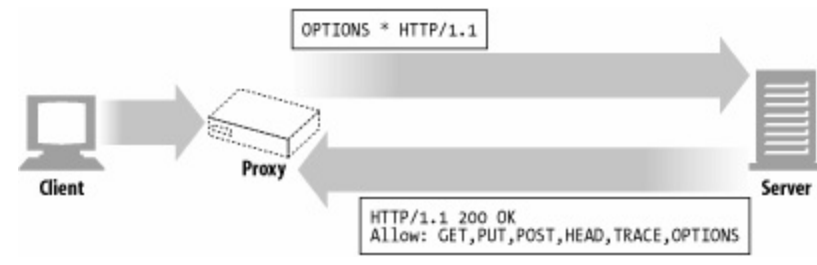
Figure 6-26. Using OPTIONS to find a server's supported methods
