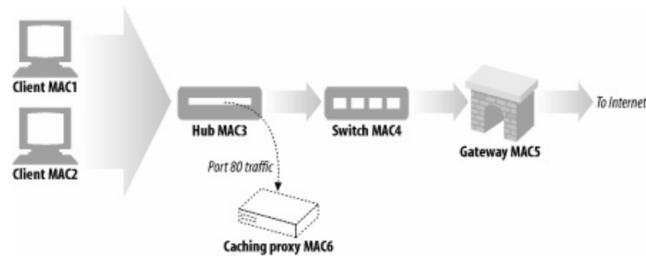
Figure 20-7. MAC forwarding using a layer-4 switch
