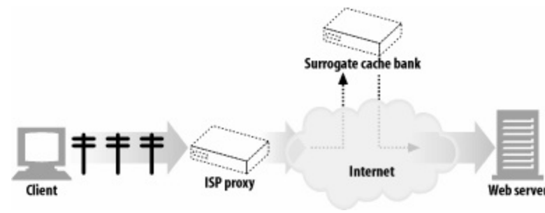
Figure 6-19. Access proxies and CDN proxies create two-level proxy hierarchies
