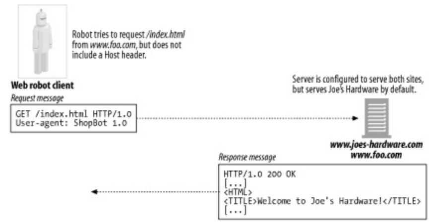
Figure 9-5. Example of virtual docroots causing trouble if no Host header is sent with the request
