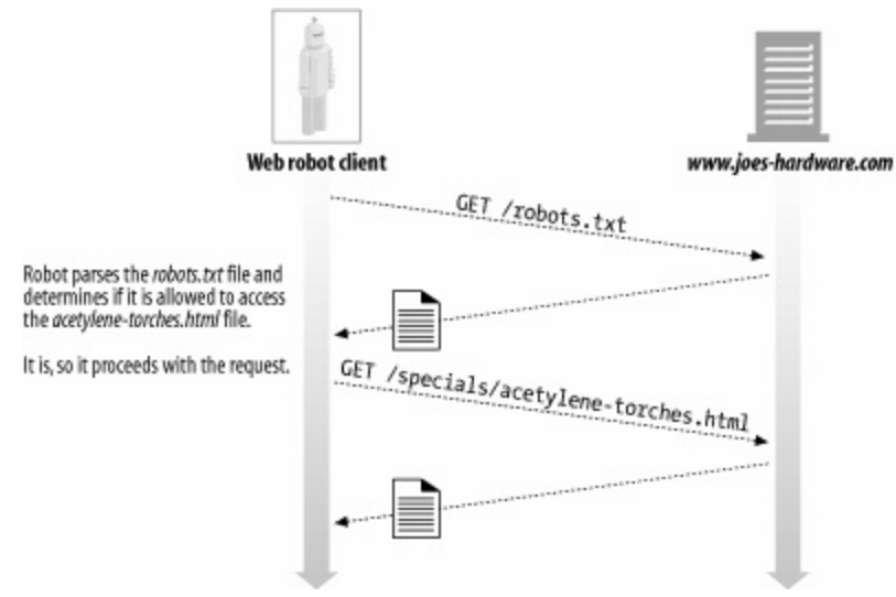
Figure 9-6. Fetching robots.txt and verifying accessibility before crawling the target file
