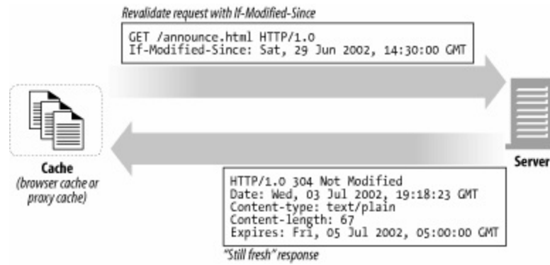
Figure 7-6. HTTP uses If-Modified-Since header for revalidation
