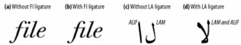
Figure 16-5. Ligatures are stylistic presentation forms of adjacent characters, not new characters
