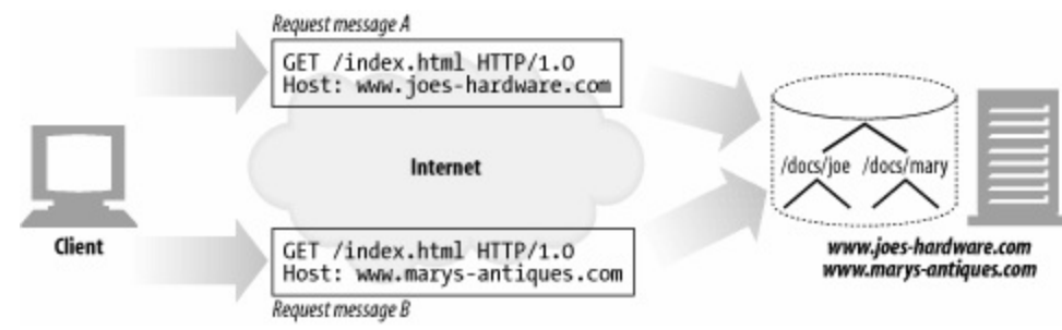
Figure 5-9. Different docroots for virtually hosted requests
