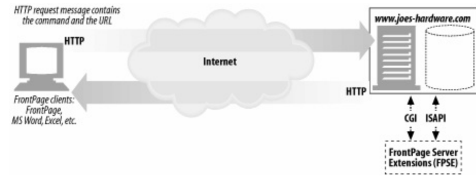
Figure 19-1. FrontPage publishing architecture
