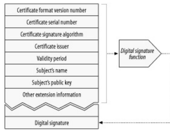
Figure 14-11. Typical digital signature format
