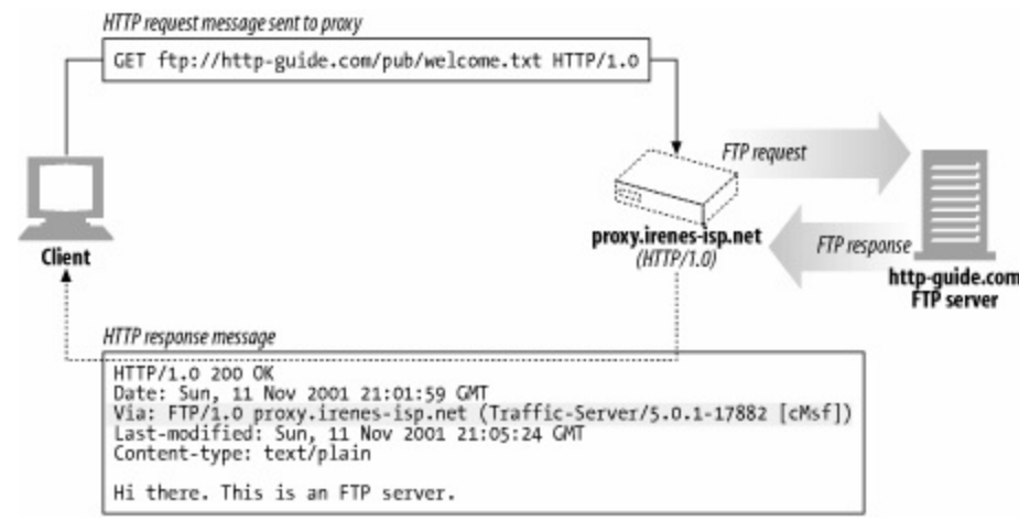
Figure 6-22. HTTP/FTP gateway generates Via headers, logging the received protocol (FTP)
