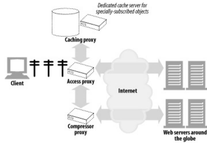
Figure 6-13. Proxy hierarchies can be dynamic, changing for each request
