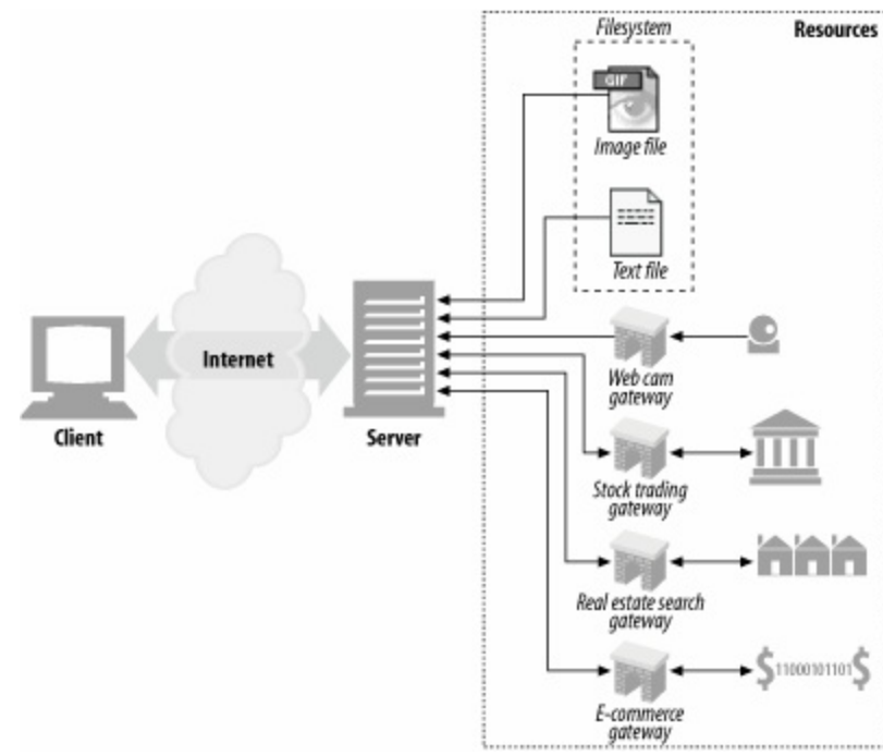
Figure 5-11. A web server can serve static resources as well as dynamic resources
