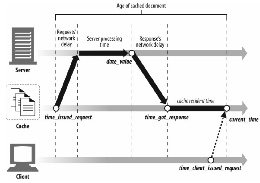
Figure 7-18. The age of a cached document includes resident time in the network and cache
