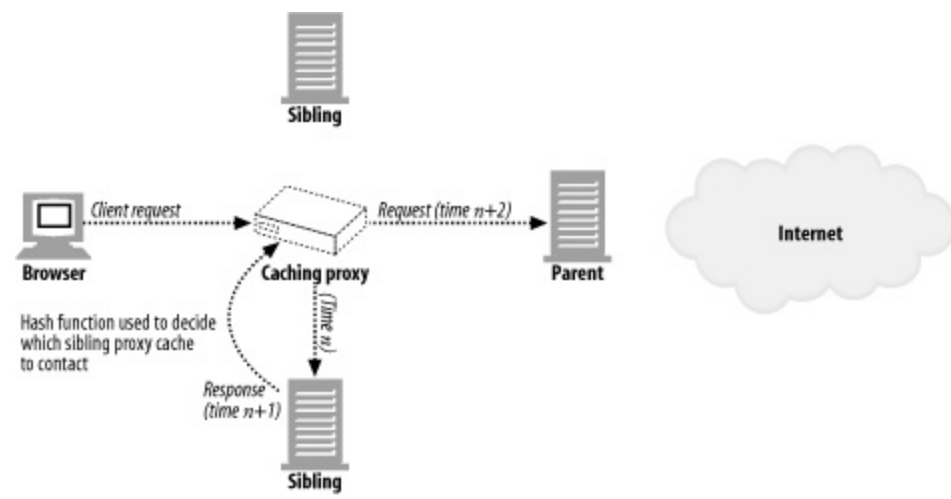
Figure 20-14. CARP redirection
