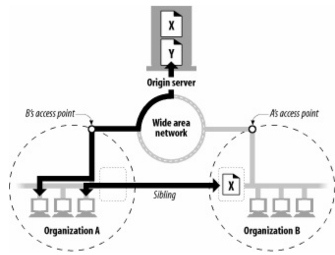
Figure 7-10. Sibling caches
