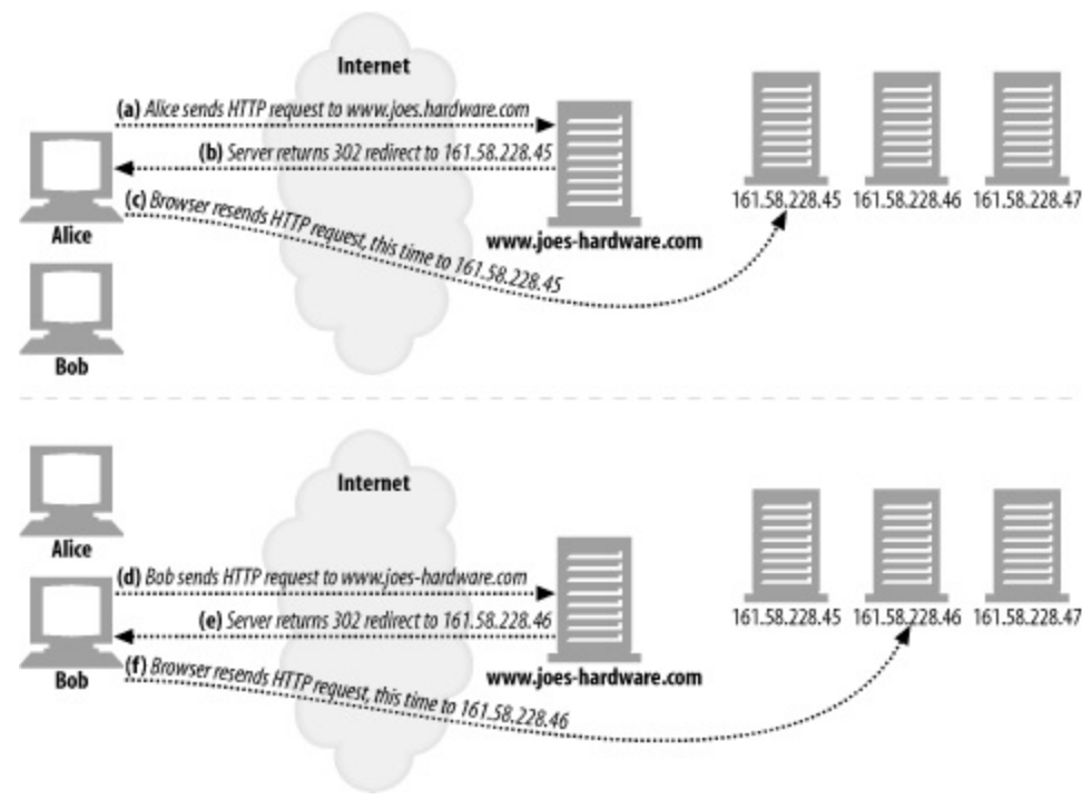
Figure 20-1. HTTP redirection
