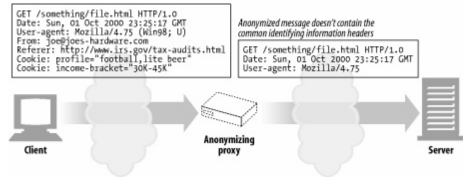
Figure 6-10. Proxy application example: anonymizer
