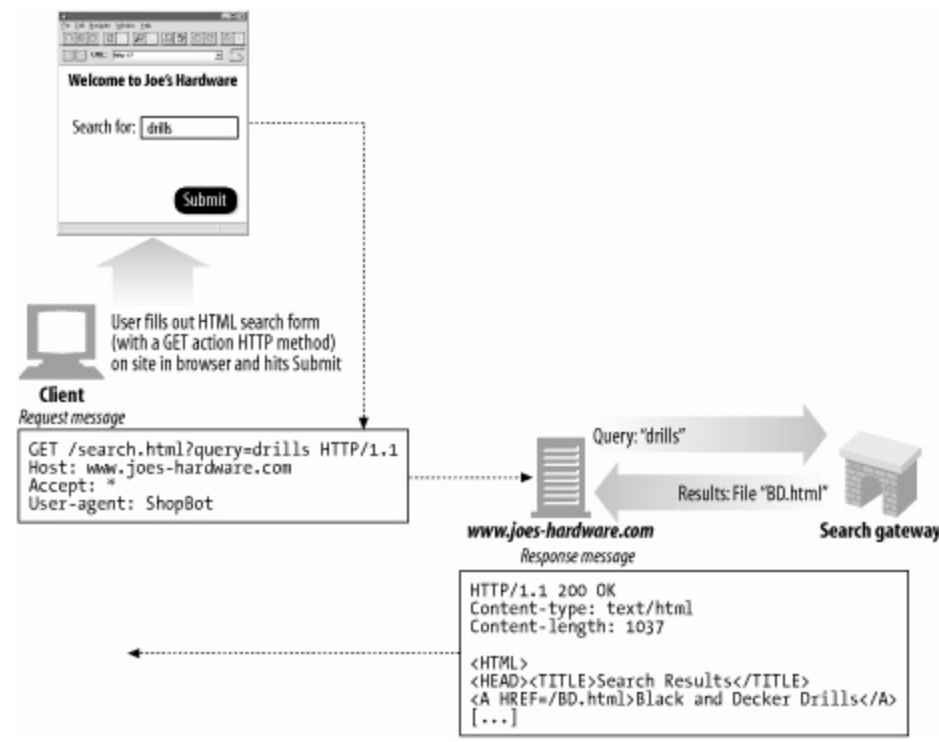
Figure 9-9. Example search query request
