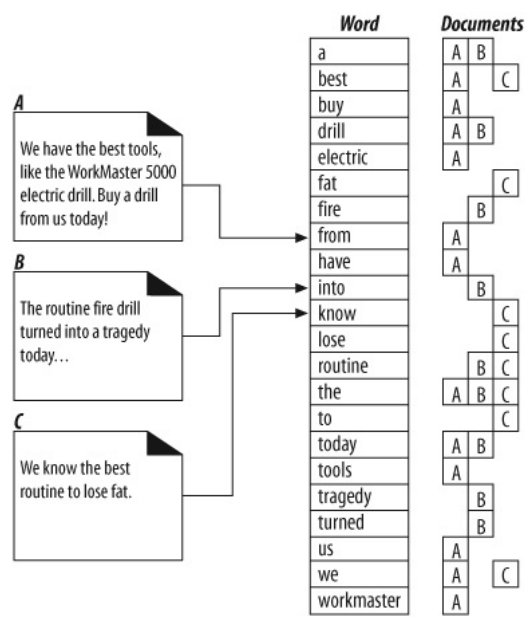
Figure 9-8. Three documents and a full-text index
