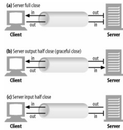
Figure 4-20. Full and half close
