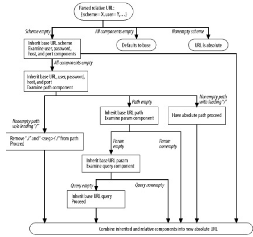
Figure 2-5. Converting relative to absolute URLs
