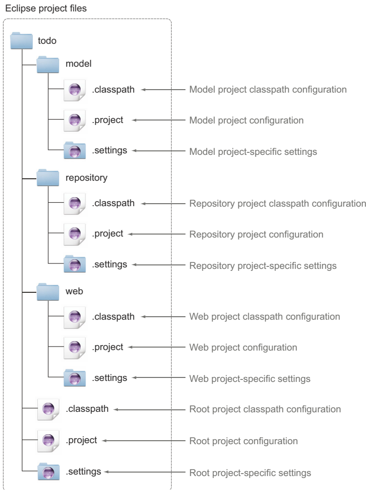
Figure 10.2 Eclipse project files
