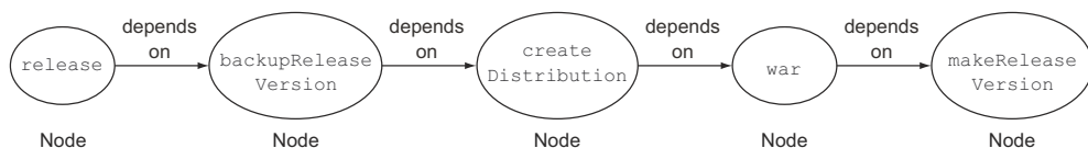
Figure 4.12 Task dependencies represented as Directed Acyclic Graph
