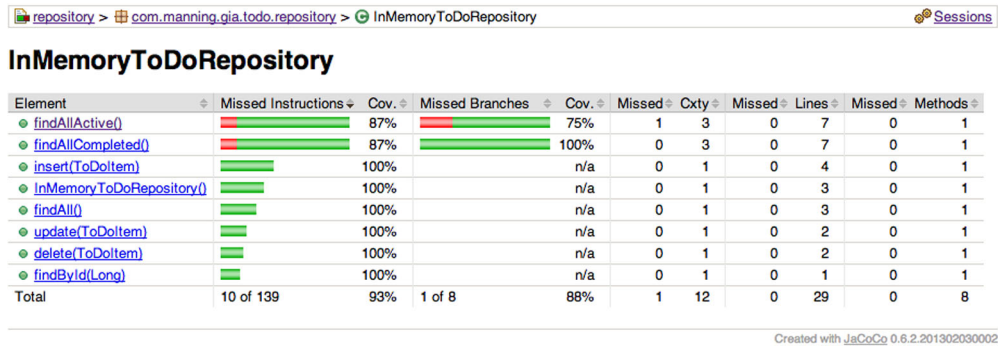
Figure 12.3 Sample JaCoCo HTML report
