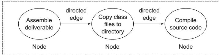
Task dependencies
