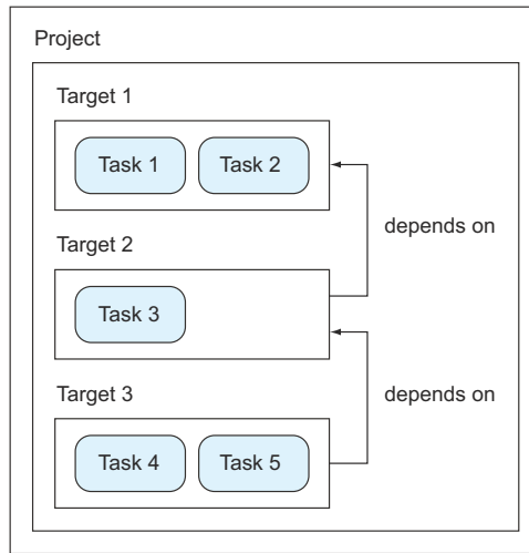
Figure 1.10 Ant's hierarchical build script structure with the elements project, target, and task
