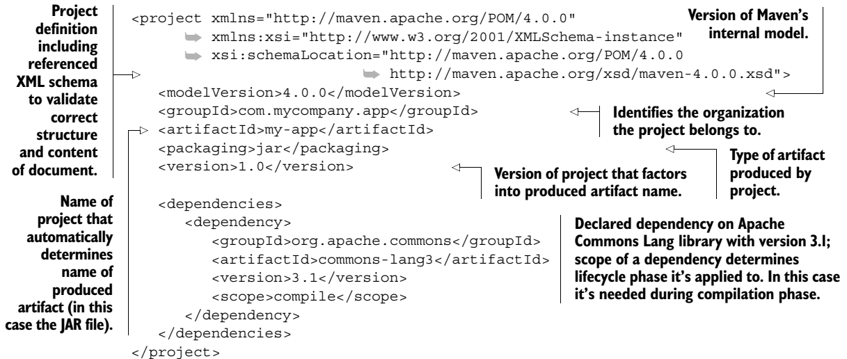
Listing 1.2 Maven POM for building standardized Java project
