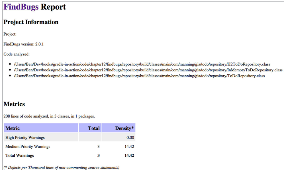
Figure 12.7 Sample FindBugs HTML report
