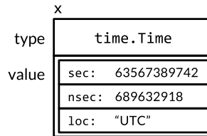
Figure 7.4. An interface value holding a time.Time struct.
