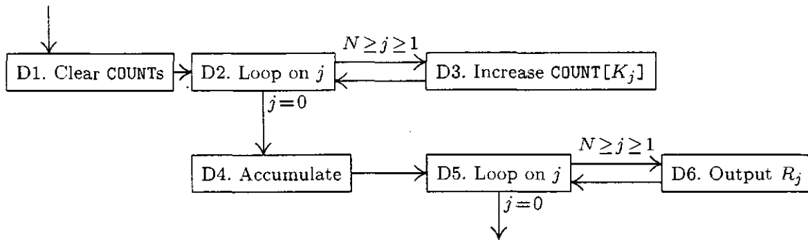
Fig. 9. Algorithm D: Distribution counting.
