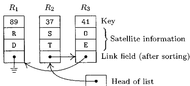
Fig. 7. List sorting.
