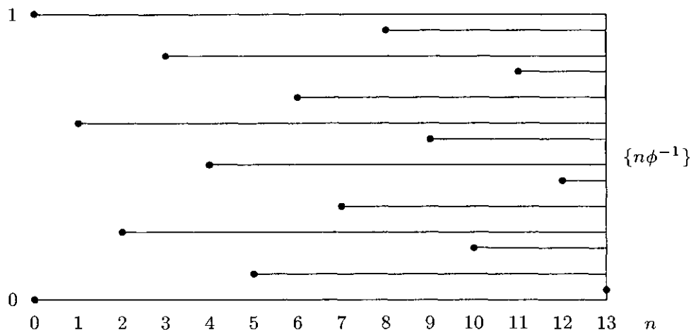
Fig. 37. Fibonacci hashing.
