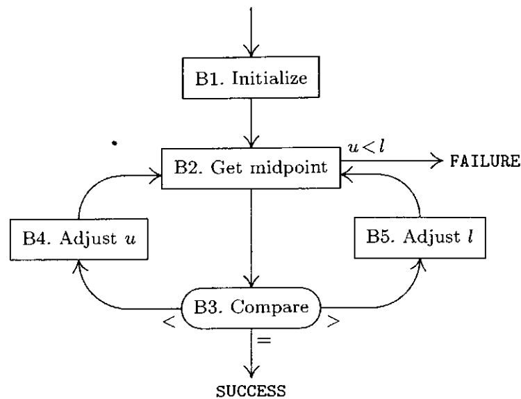
Fig. 3. Binary search.
