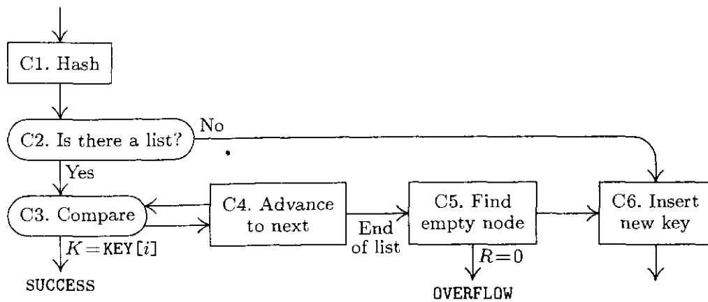
Fig. 39. Chained hash table search and insertion.
