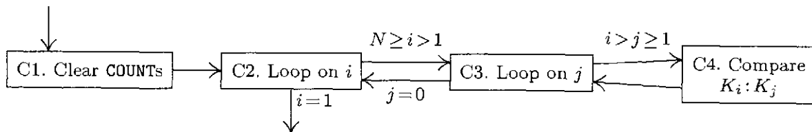
Fig. 8. Algorithm C: Comparison counting.
