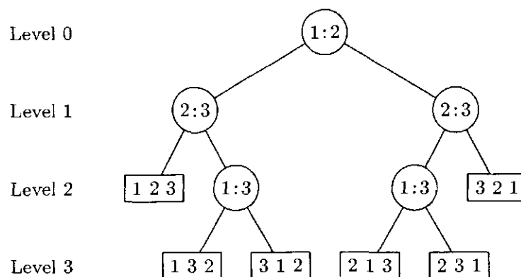
Fig. 34. A comparison tree for sorting three elements.
