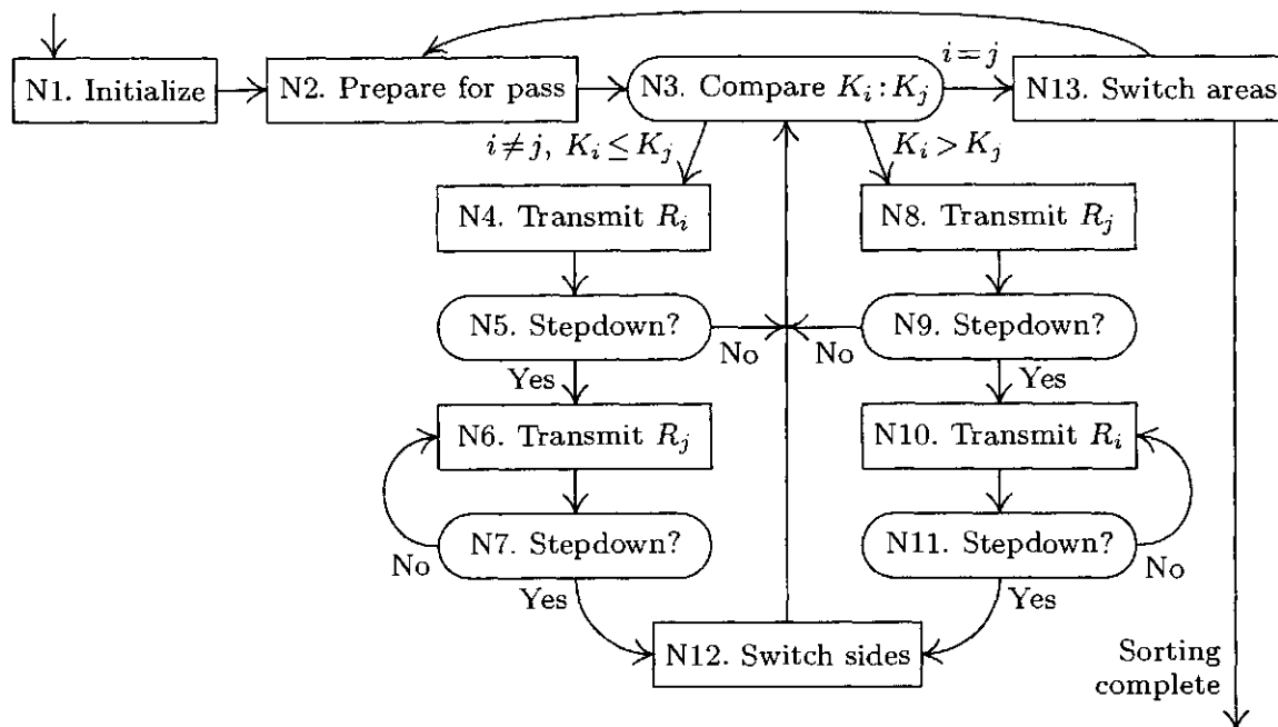
Fig. 30. Merge sorting.
